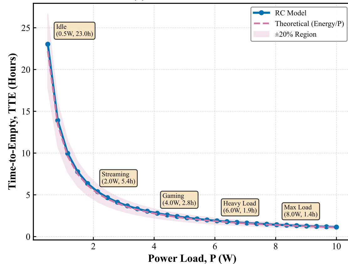
(a) TTE vs. Power Load
