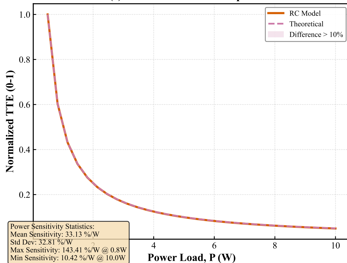
(c) Normalized TTE Comparison
