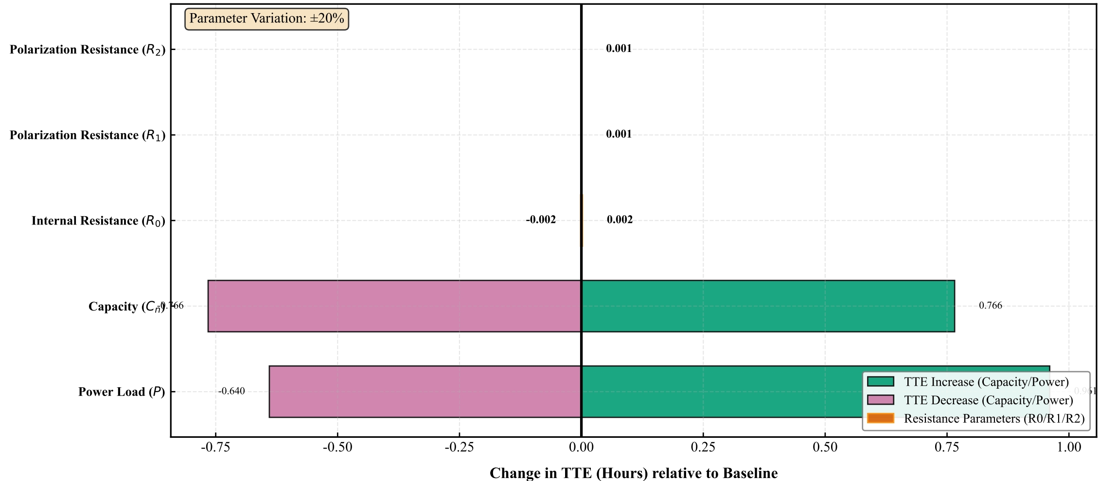
Tornado Plot: Parameter Sensitivity Analysis for TTE (Baseline: 3.0W Constant Power, TTE = 3.83h)
