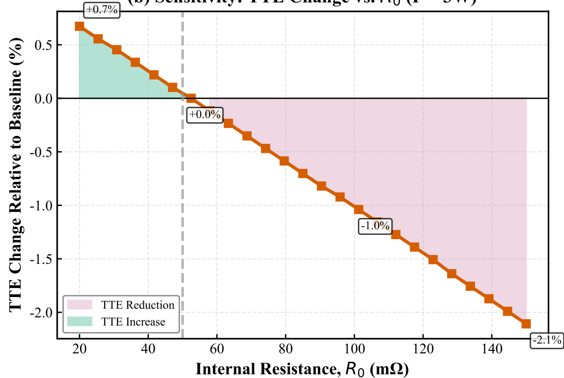
(b) Sensitivity: TTE Change vs. R_0 ( P = 3 W)
