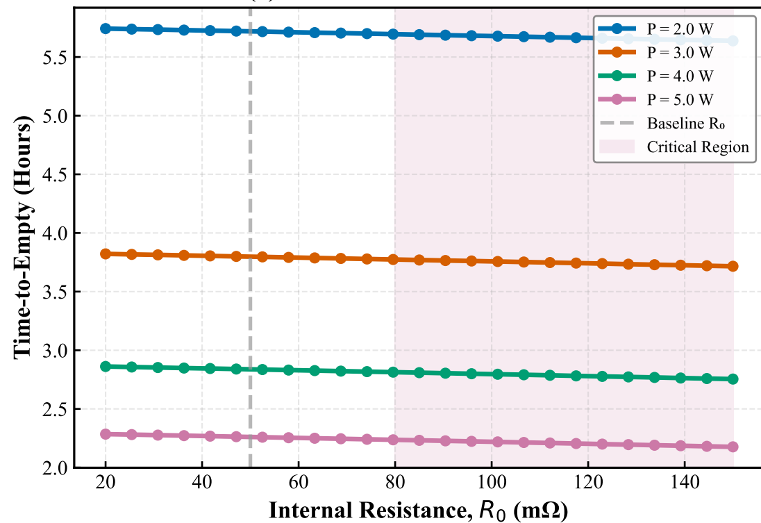
(a) TTE vs. Internal Resistance
