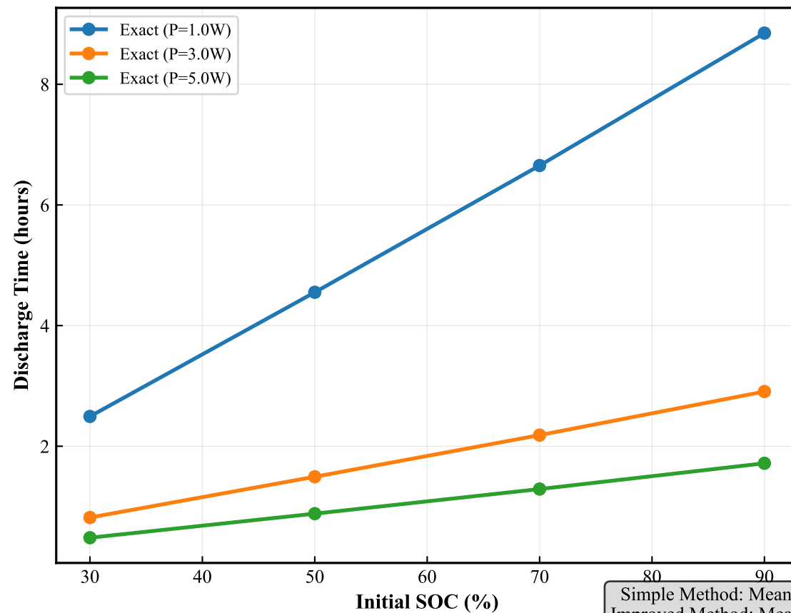
Exact Solution: Time vs SOC
