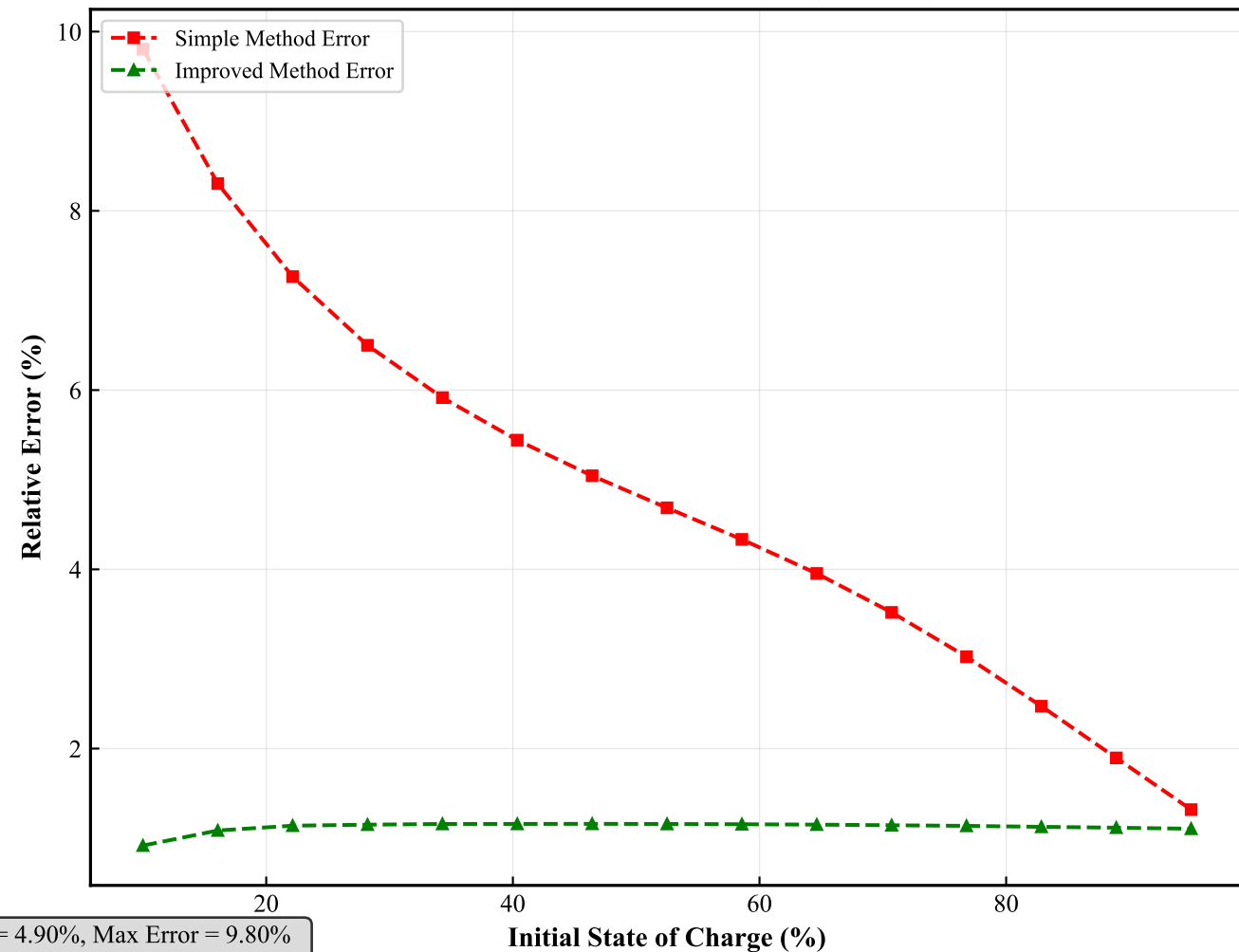
Prediction Error vs Initial SOC (P=3.0 W)
