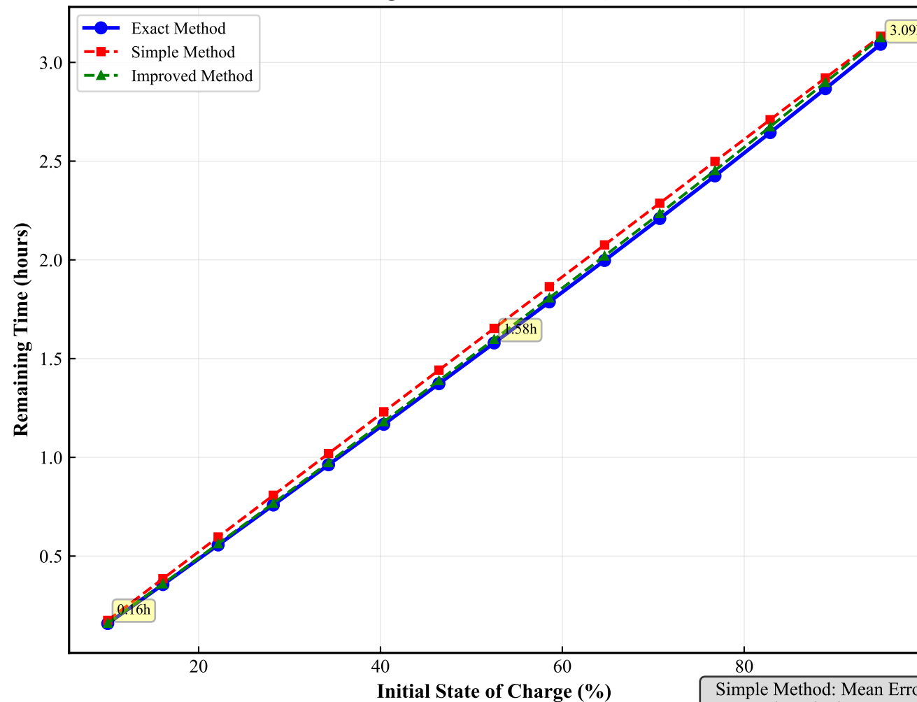
Remaining Time vs Initial SOC (P=3.0 W)
