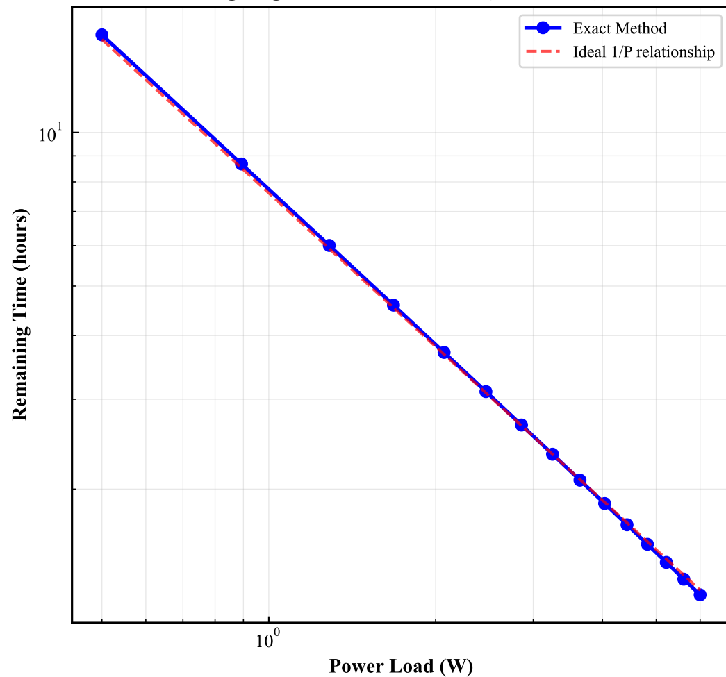
Log-Log Plot: Time vs Power (SOC=80%)
