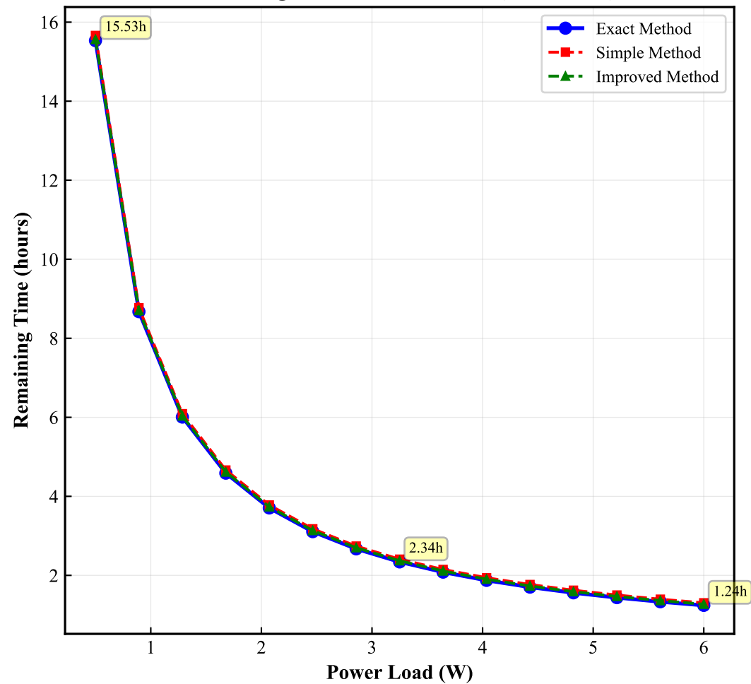
Remaining Time vs Power Load (SOC=80%)
