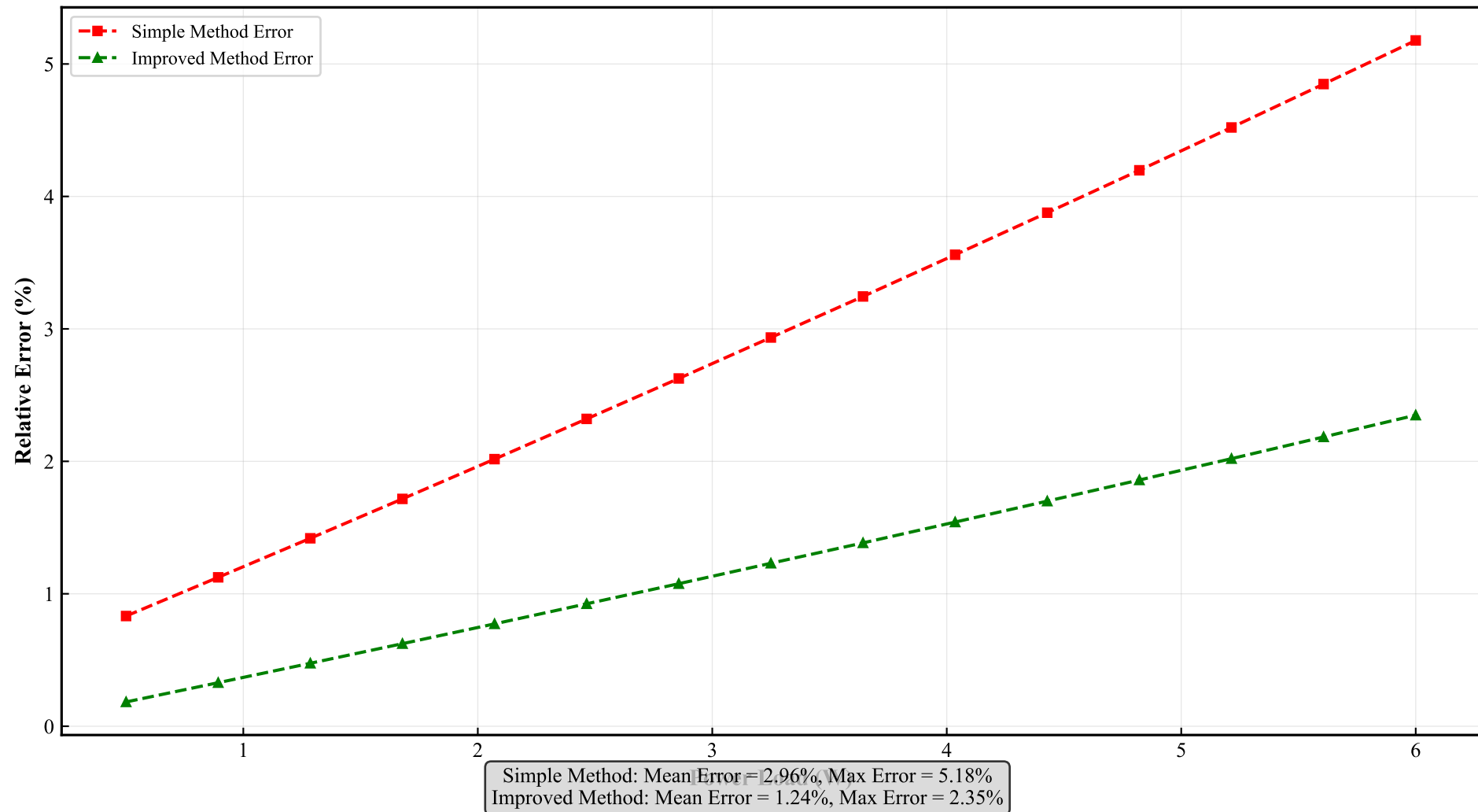
Prediction Error vs Power Load (SOC=80%)
