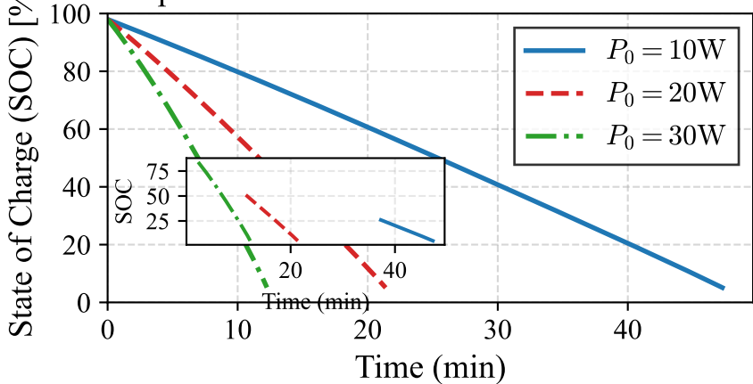
SOC Depletion Curves under Constant Power Discharge
