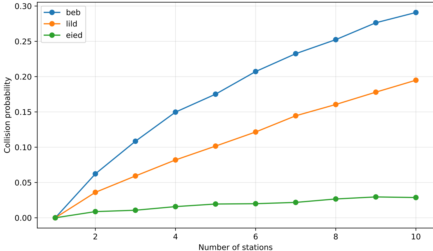
Collision Probability vs Number of Stations
