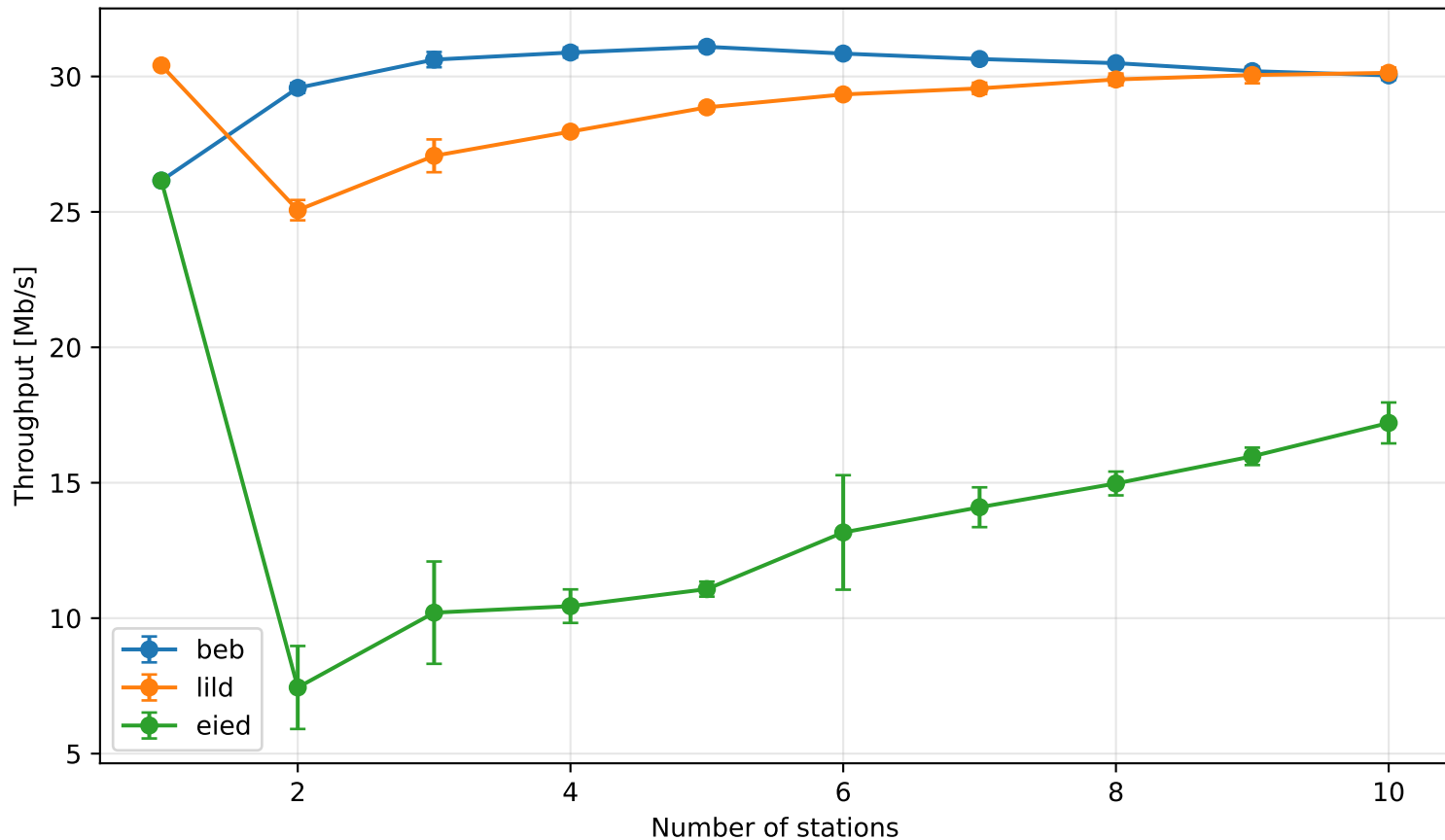
Throughput vs Number of Stations
