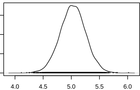
Density of \mu[2]
