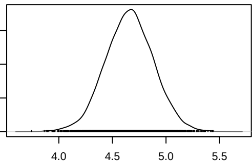
Density of \mu[3]
