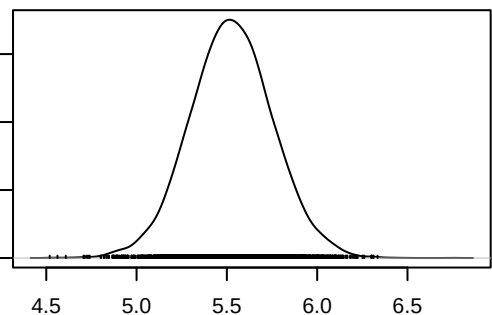
Density of \sigma
