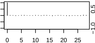
lam[3]
