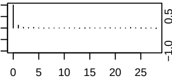
lam[2]
