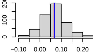
Histogram of \phi_{\text{sample}5}
