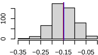
Histogram of \phi_{\text{sample}7}
