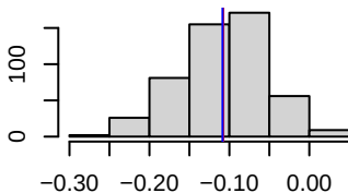
Histogram of \phi_{\text{sample}8}
