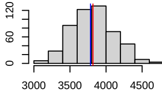
Histogram of v
