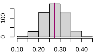
Histogram of \phi_{\text{sample}4}
