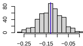
Histogram of \phi_{\text{sample}6}
