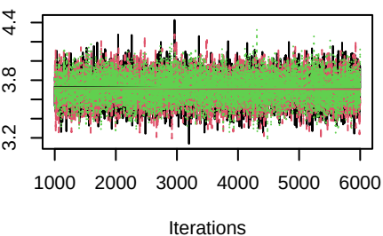
Trace of \mu[1,1]
