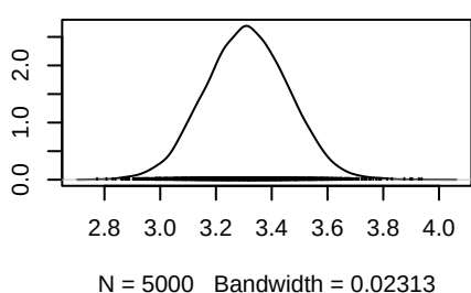
Density of \mu[2,2]
