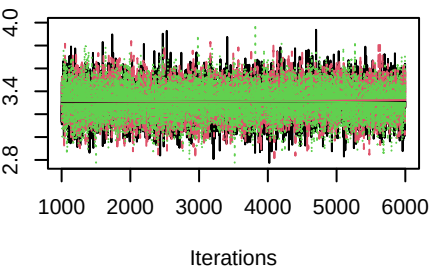
Trace of \mu[2,2]
