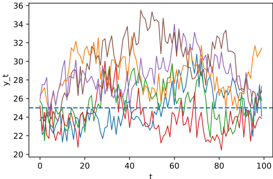
Constant DLM \{1,1,1,W\} with W = 0.5
