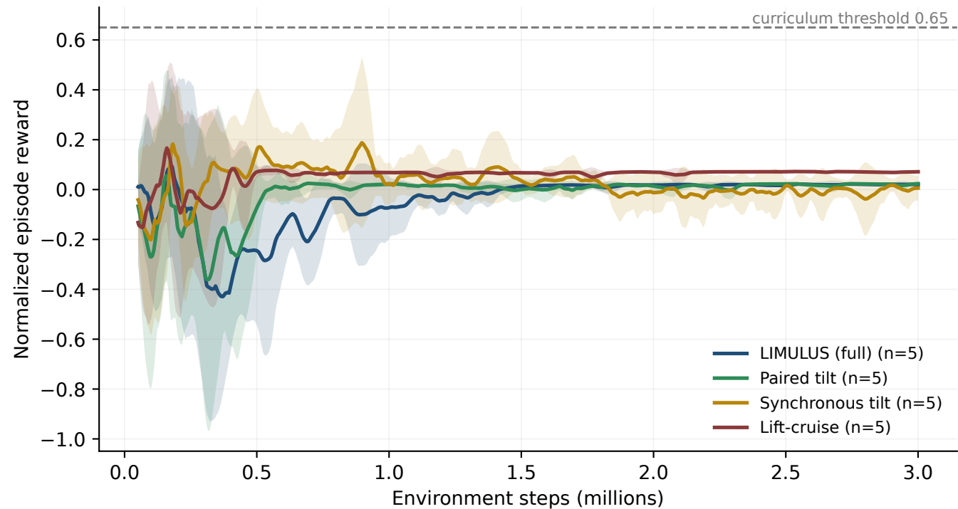
Training reward, mean of five seeds with \pm 1 SD band
