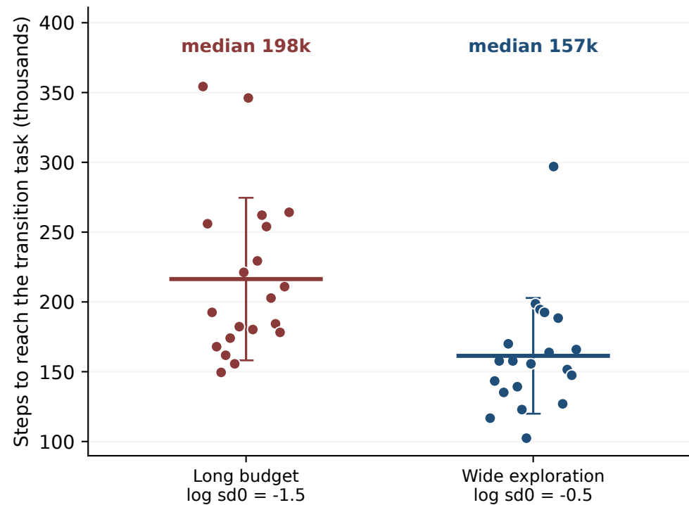
Arrival at the transition task
