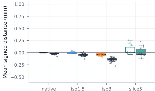
Expert mask
