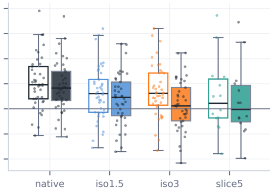
TotalSegmentator fast
