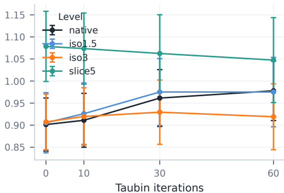
TotalSegmentator fast
