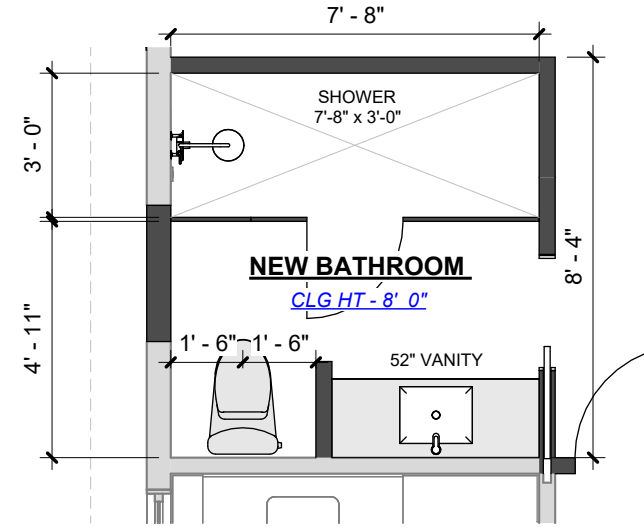
3 Proposed - Second floor OP#B 1/4" = 1'-0"
