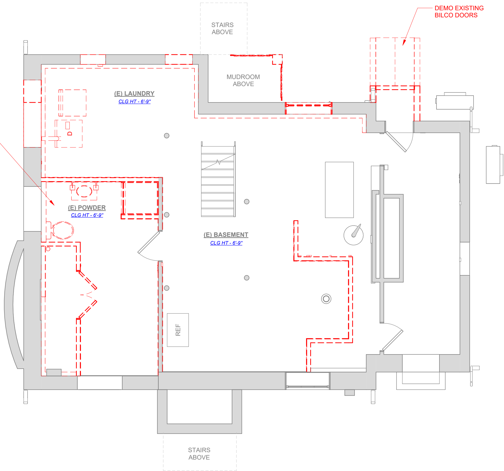
① Existing - Basement Floor. 1/4" = 1'-0"
