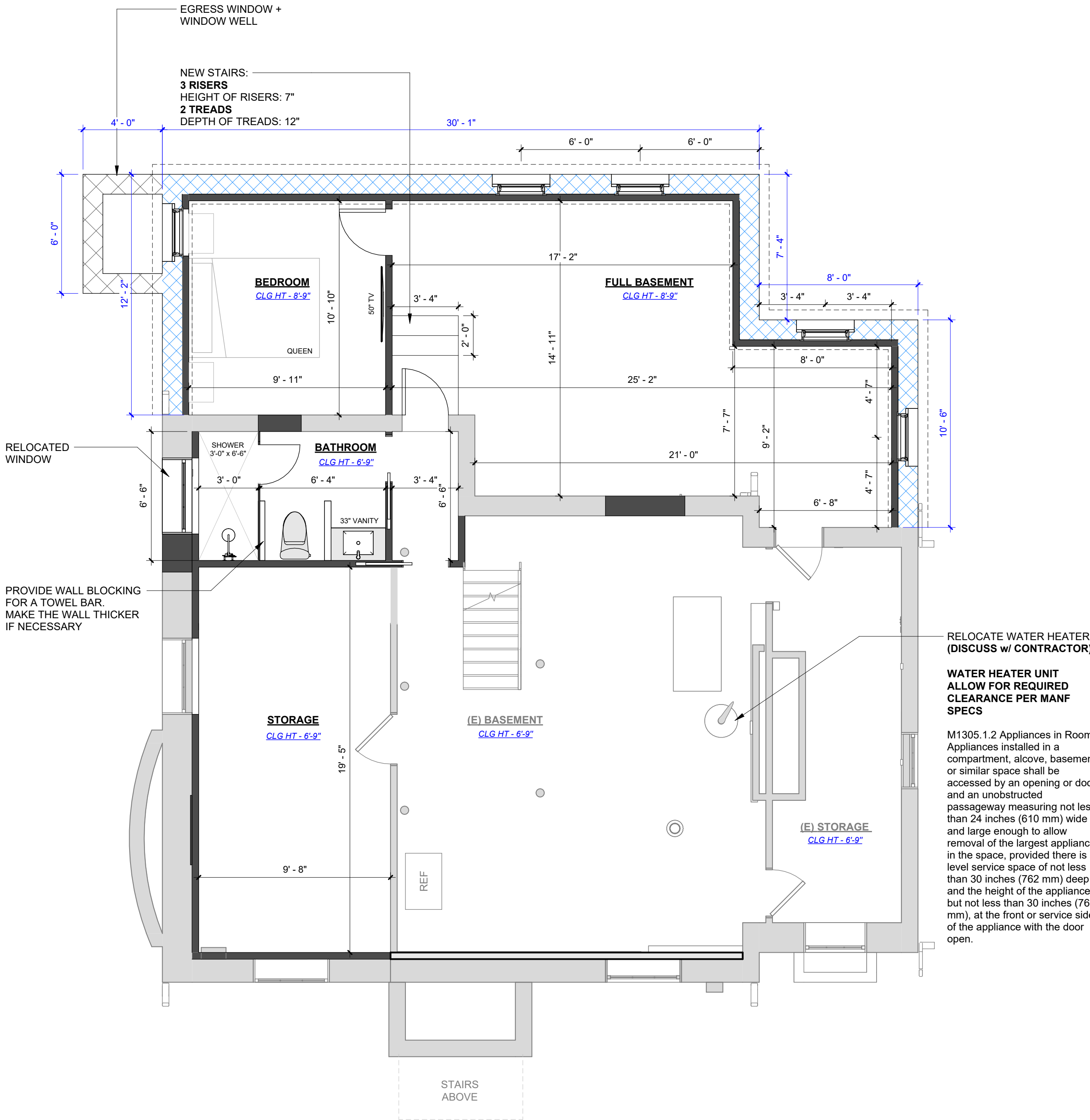
② Proposed - Basement Floor. 1/4" = 1'-0"
