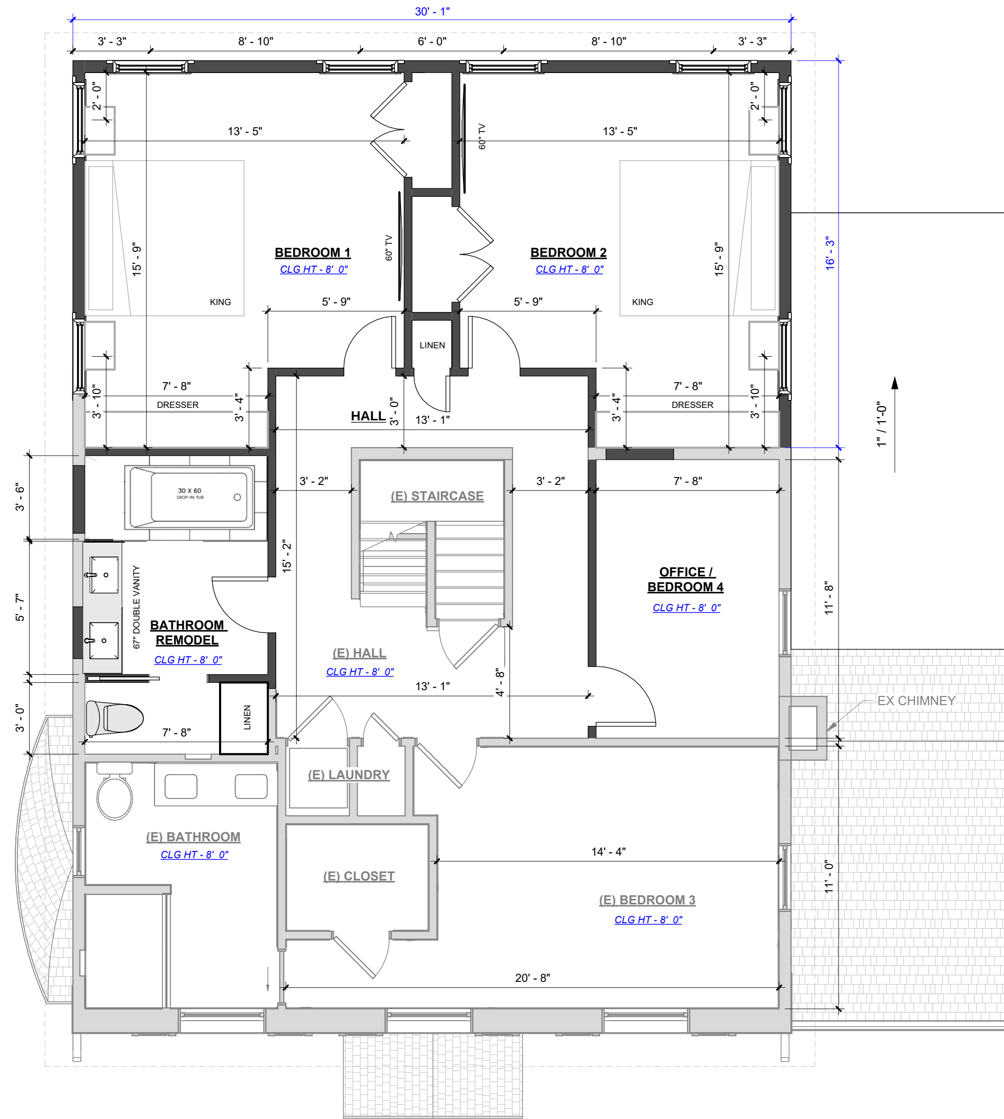
3 Proposed - Second floor OP#B 1/4" = 1'-0"
