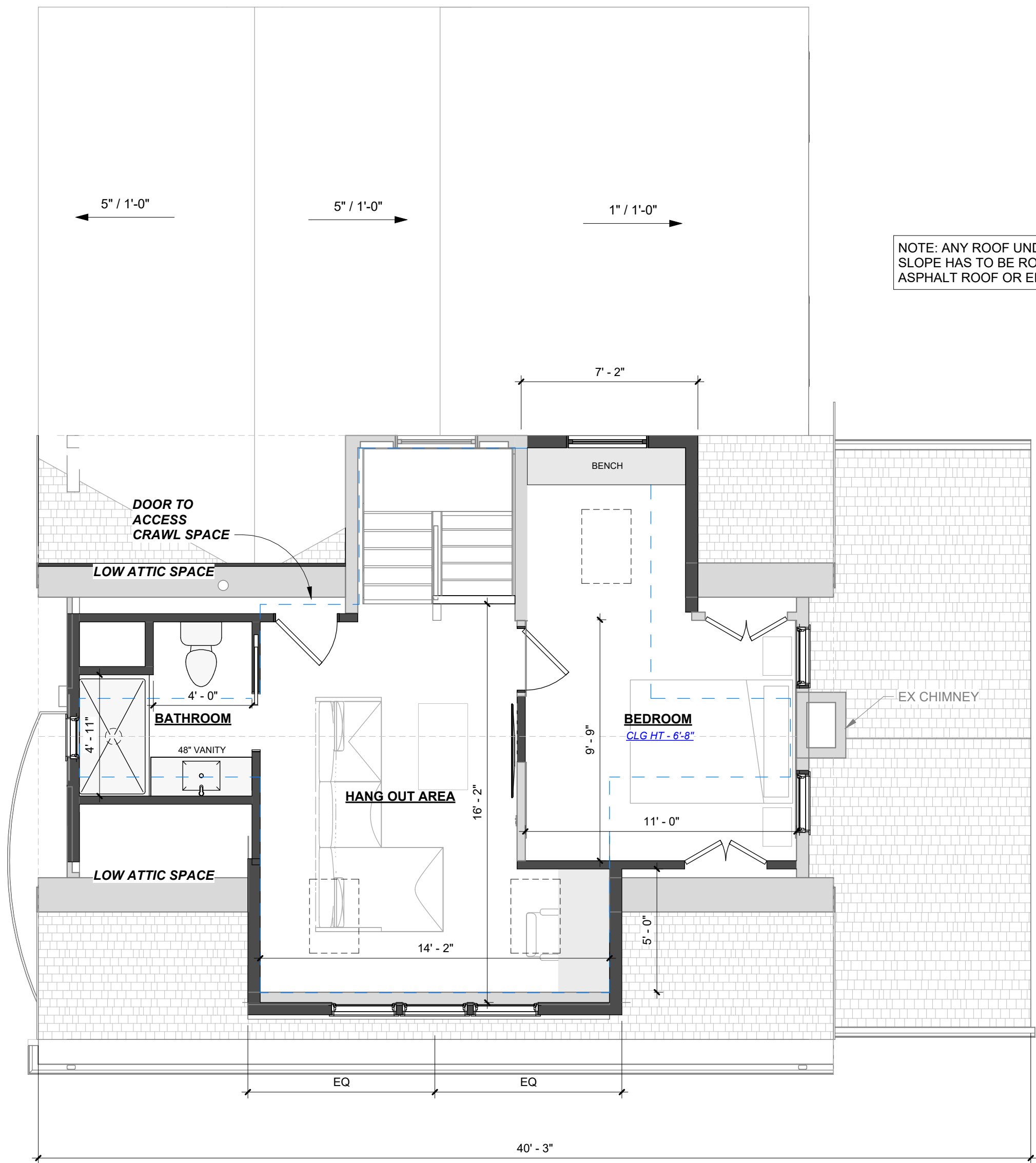
2 Poposed - Third floor 1/4" = 1'-0"
