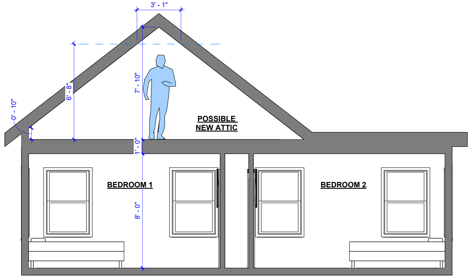
3 Building Section - OP #B 1/4" = 1'-0"
