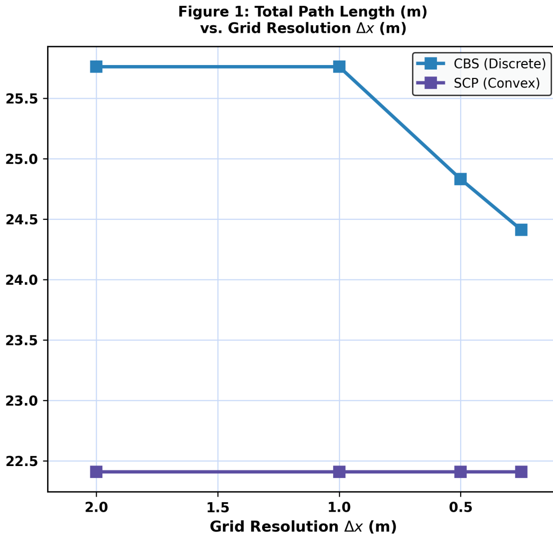
Figure 1: Total Path Length (m) vs. Grid Resolution \Delta x (m)
