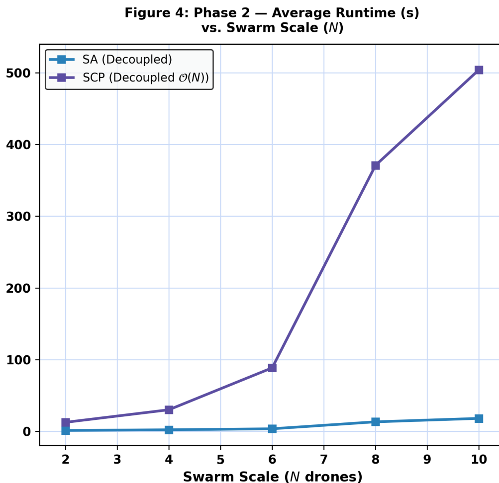
Figure 4: Phase 2: Computational Runtime vs. Swarm Scale
