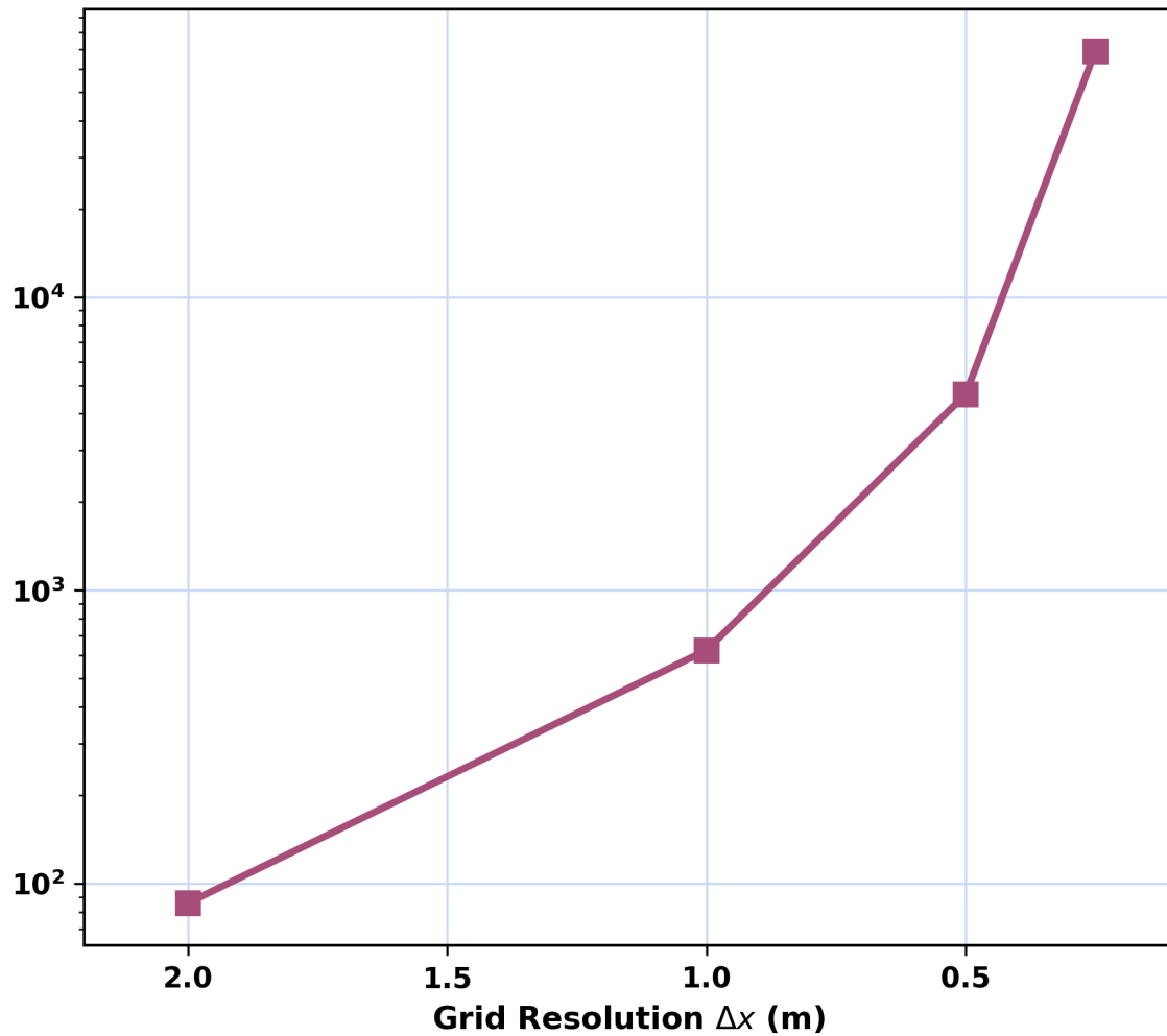
Figure 2: A* Nodes Expanded (Log Scale) vs. Grid Resolution \Delta x (m)
