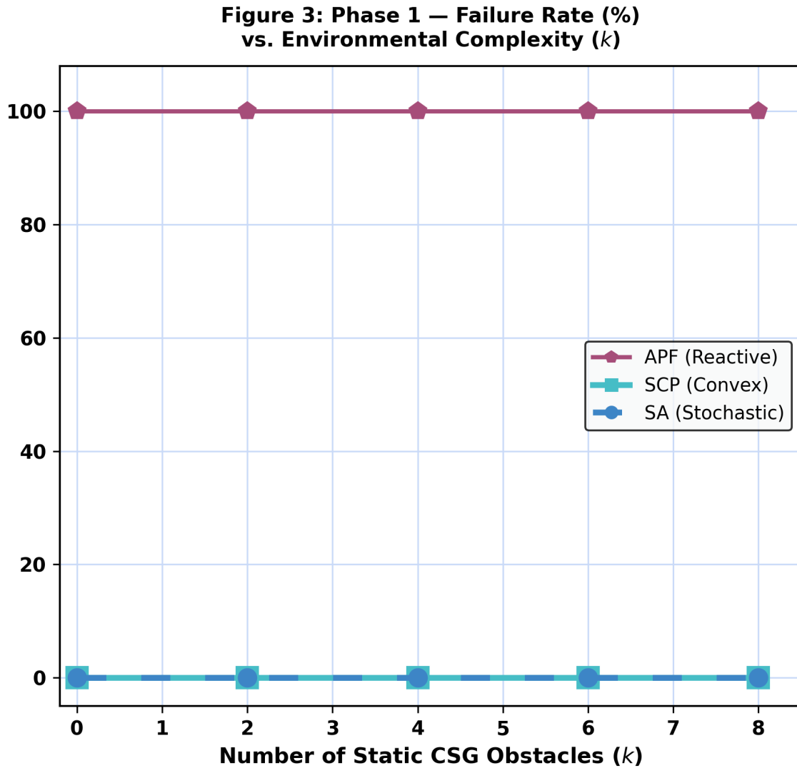
Figure 3: Phase 1: Collision/Failure Rate vs. Environmental Complexity
