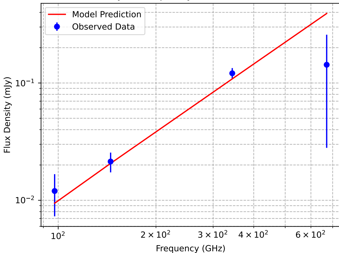
Flux Density vs Frequency for CPD around PDS 70 c
