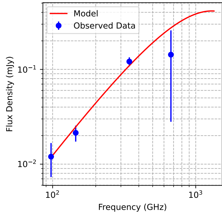
Dusty Ring model T=22.02 K
