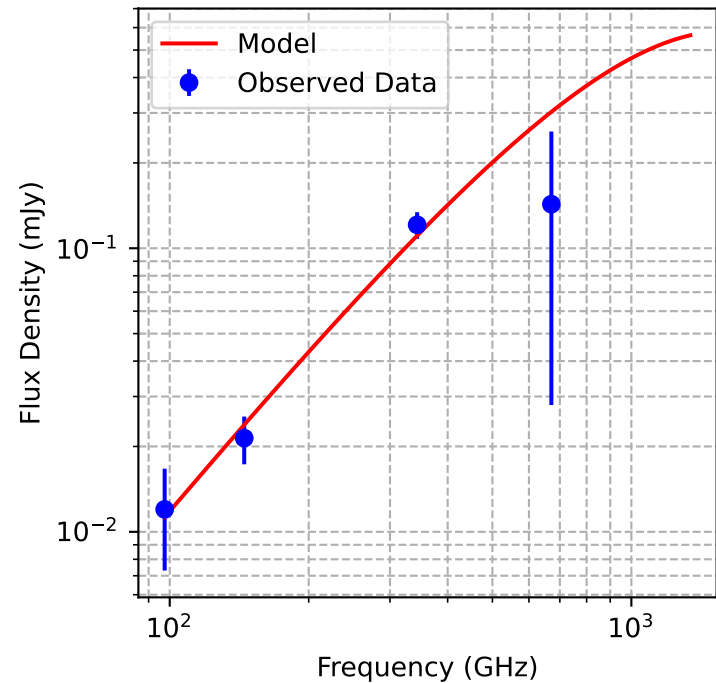
Dusty Ring model T=27.0 K
