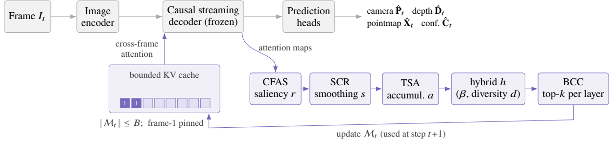
Figure 1. Overview of Keep3R. Each incoming frame is encoded and decoded causally against a bounded KV cache, yielding per-frame camera parameters, depth, pointmap, and confidence. The cross-frame attention of the current frame provides a saliency signal for every cached token (CFAS), which is smoothed over the source patch grid (SCR) and accumulated over time (TSA). Budgeted cache compression (BCC) fuses the accumulated importance with a diversity score, allocates the budget across layers, and retains the top-scoring tokens, with the reference frame pinned, so that the cache never exceeds B tokens.
