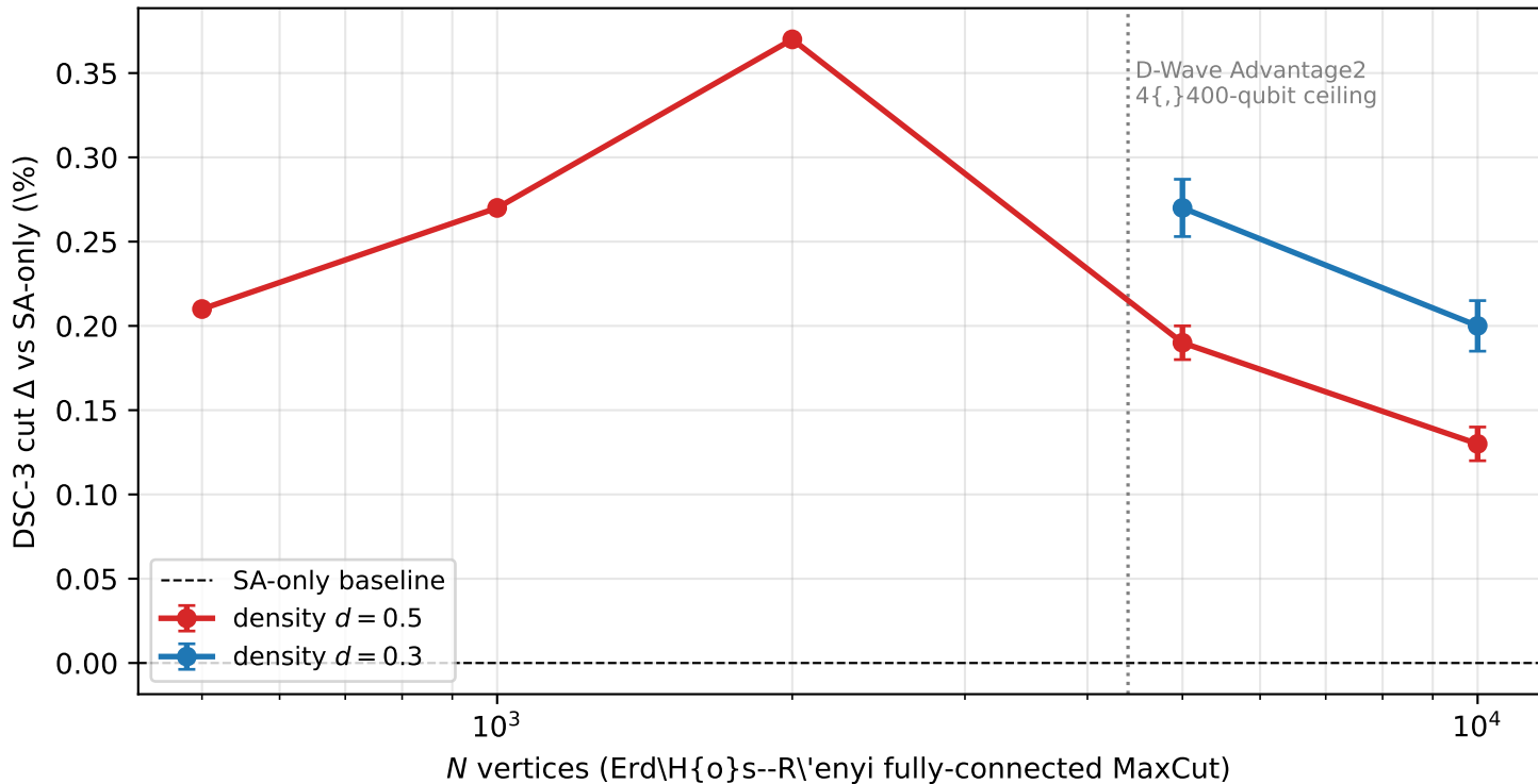
B3 MaxCut crossover persists past the D-Wave embedding ceiling
