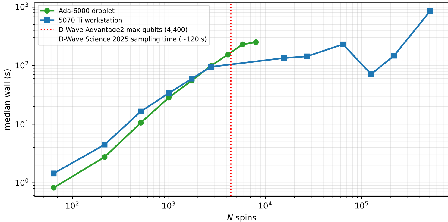
DSC-3 ceiling push: wall-time scaling well past D-Wave's embedding limit
