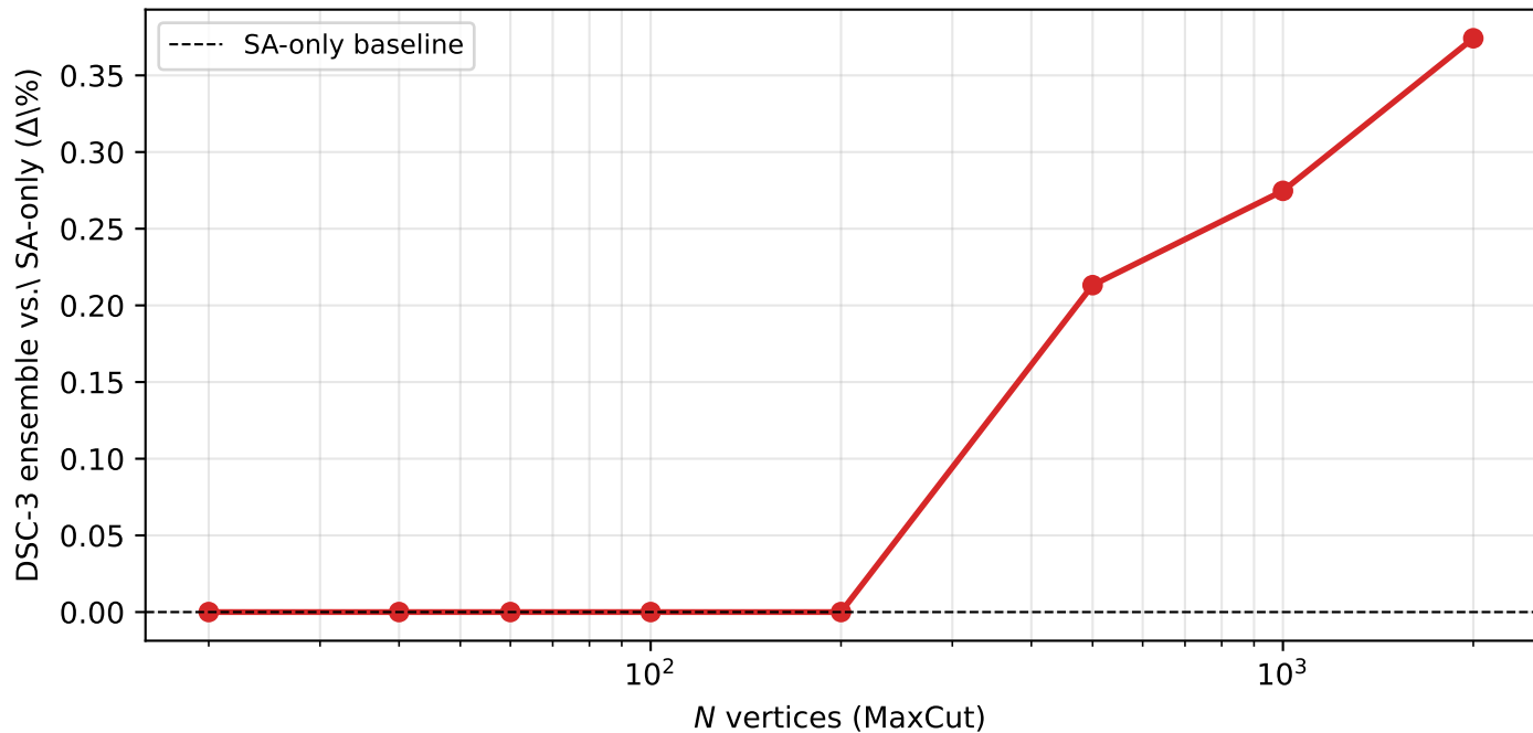
B3 MaxCut: ensemble advantage grows with problem size
