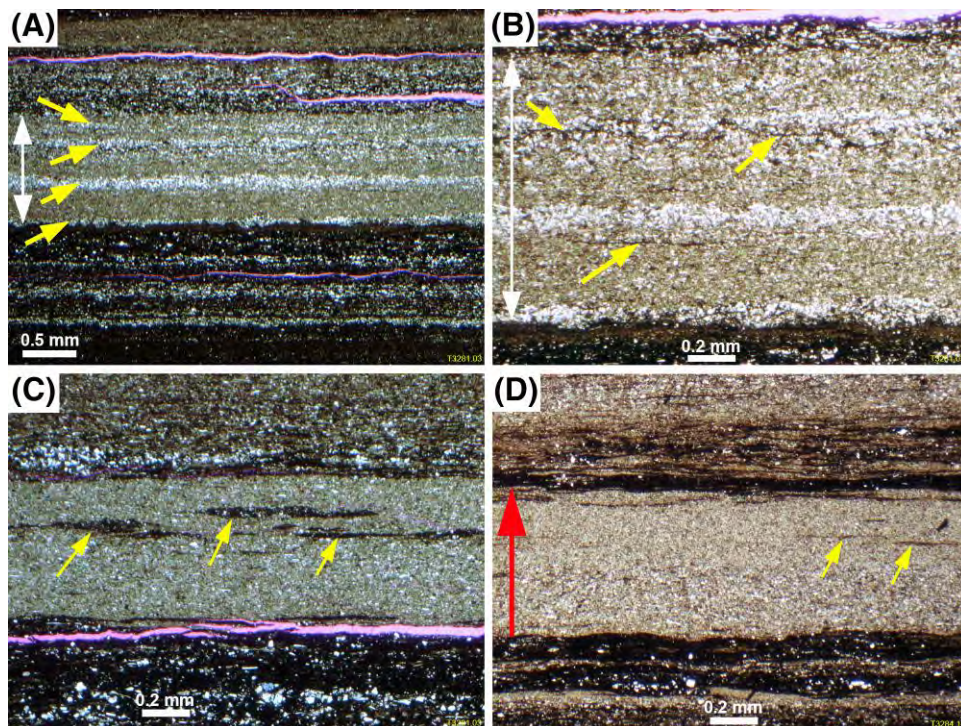
Figure 17. Photomicrographs showing sedimentary features of clay drapes within facies CS1 (striped carbonaceous shale) (Tanumbirini-1). (A) Clay drape with thin silt laminae (yellow arrows). (B) Close-up view of (A). Silt laminae vary in thickness laterally and consist of small adjoining lenses. Thin carbonaceous streaks (yellow arrows) are common. (C) Clay drape with well-developed dark carbonaceous streaks (yellow arrows). Internally these streaks are texturally identical to wavy-anastomosing carbonaceous laminae (Figure 12). (D) Clay drape with subtle vertical grading (red arrow), due to a higher content of silt grains in the lower half. It also contains dark carbonaceous streaks (yellow arrows) as seen in (C).
