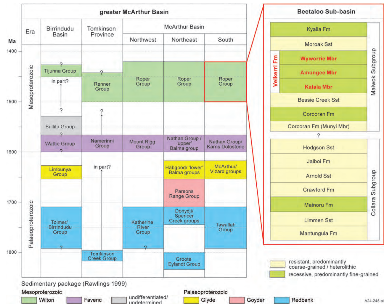
Figure 3. Group level correlation chart for the greater McArthur Basin showing stratigraphic packages of Rawlings (1999) and Close (2014), and Beetaloo Sub-basin Roper Group stratigraphy with Velkerri Formation members highlighted in bold red text (modified from Jarrett et al., 2022). Color coding for packages is same as in Figure 1. Fm = Formation; Mbr = Member; Sst = Sandstone.
