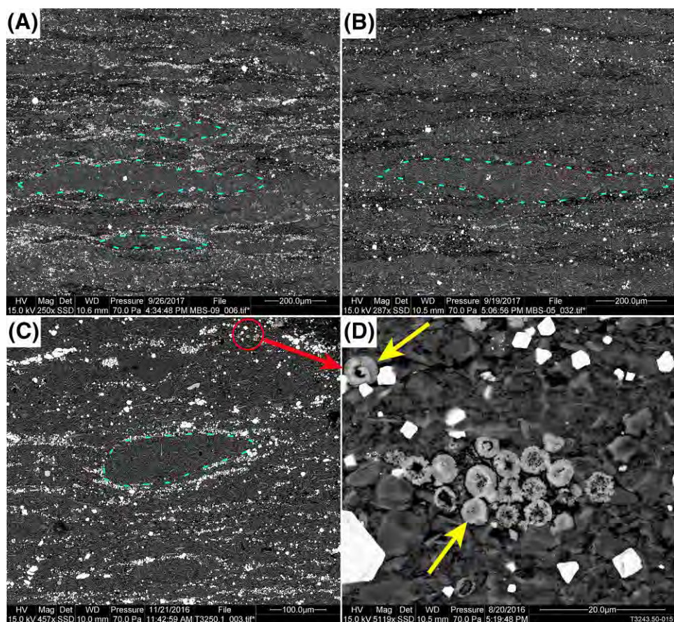
Figure 14. (A–C) SEM (scanning electron microscope) backscatter images from homogenous-lenticular carbonaceous laminae show petrographically distinct deformed-flattened lenticles (some examples outlined with dashed blue line) that are surrounded-bordered by a pyrite-rich (bright grains) matrix. The red circle marks typical matrix, and (D) shows matrix composition and texture at higher magnification with dispersed organic matter (black), pyrite grains (bright), and scattered and clustered phosphate spheres (yellow arrows). (A) and (B) are from Marmbulligan-1, (C) and (D) are from Tanumbrini-1.
