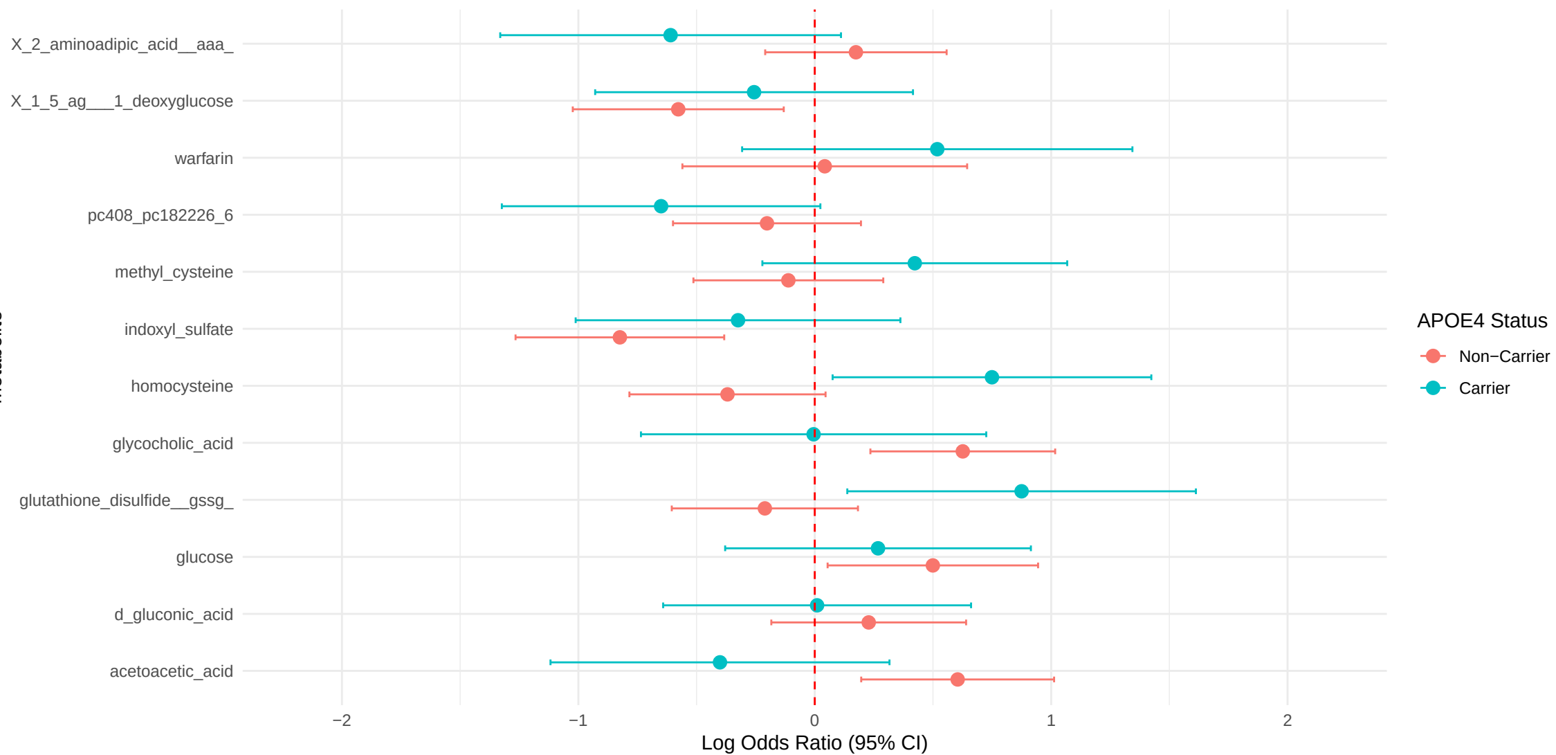
Combo w/ Metabolite–APOE4 Stratified Interaction
