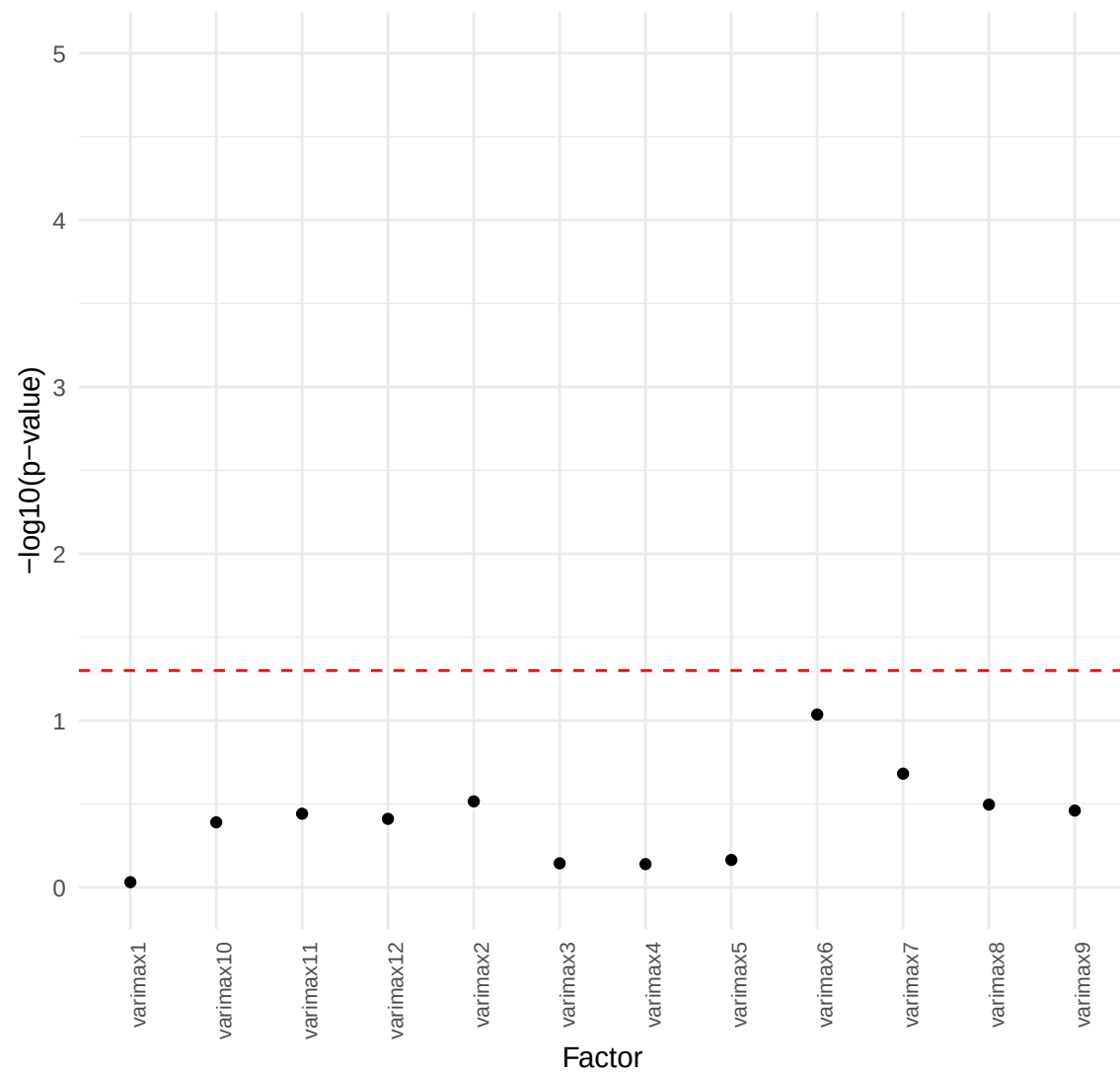
Varimax Manhattan Plot (EA w/ APOE4 Covariate)
