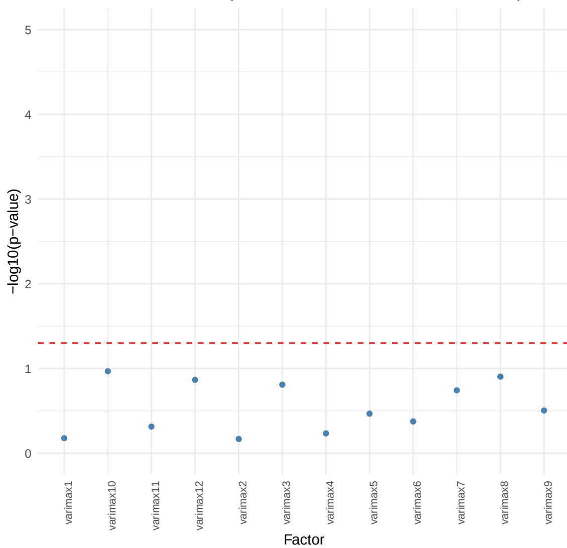
Varimax Manhatta Plot (AA w/ Metabolite-APOE4 Interaction)
