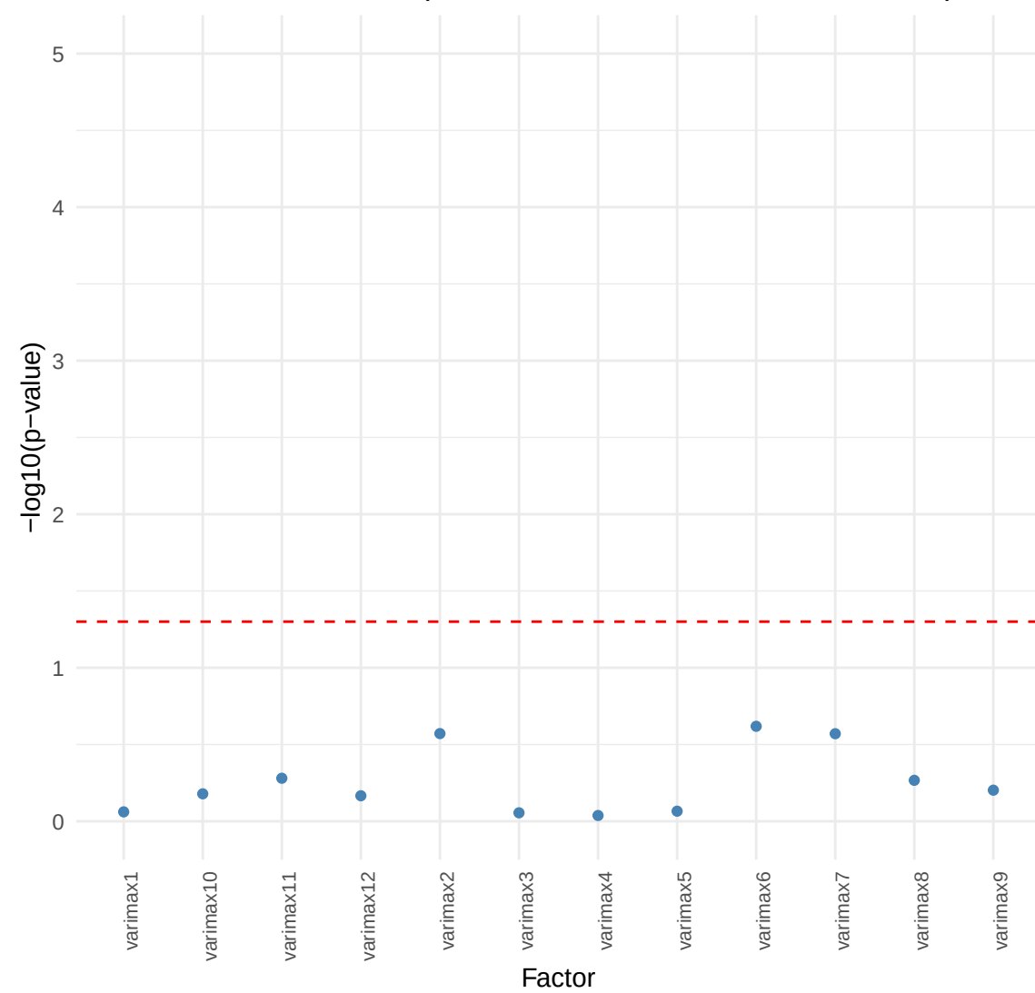
Varimax Manhatta Plot (EA w/ Metabolite-APOE4 Interaction)
