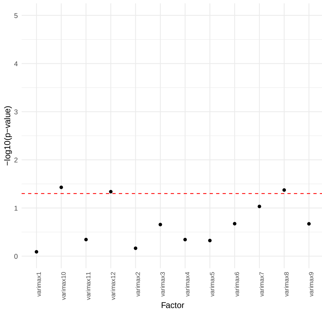
Varimax Manhattan Plot (AA w/ APOE4 Covariate)
