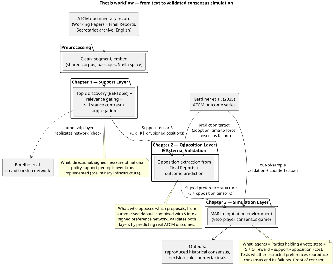
Figure 2.1: Thesis workflow: from the ATCM documentary record to a validated consensus simulation. The support layer (Chapter 1) produces a signed position tensor S ; the opposition layer (Chapter 2) adds an opposition tensor O and validates both against ATCM outcomes; the simulation layer (Chapter 3) tests whether the extracted preferences reproduce consensus and its failures.
