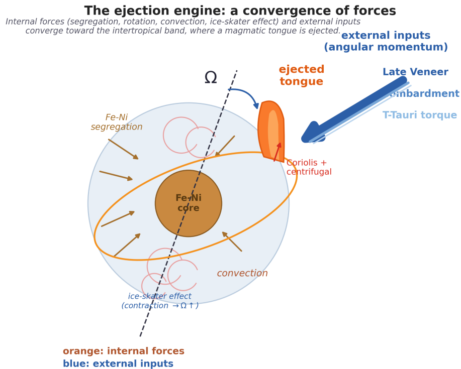
Figure 2: The ejection engine: a convergence of forces. Internal forces (Fe-Ni segregation toward the core, rotation \Omega , convection, ice-skater effect: contraction \rightarrow \Omega \uparrow ) and external angular-momentum inputs (Late Veneer, bombardment, T-Tauri torque) converge toward the intertropical band, where a magmatic tongue is ejected under the combined action of the Coriolis and centrifugal forces. Orange: internal forces; blue: external inputs.
