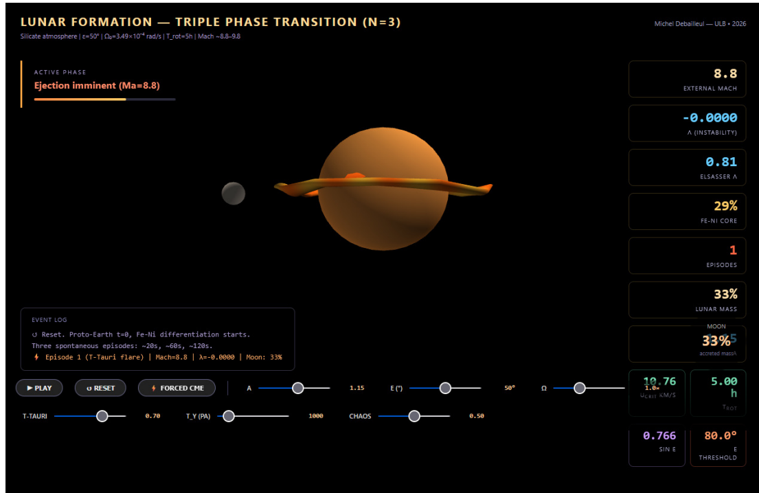
Figure 4: Screenshot of the interactive simulation accompanying this work (link above), showing the Coherent Magmatic Torus (CMT) during ejection around the proto-Earth, with the real-time dynamic parameter dashboard (external Mach number, \lambda instability, Elsassers number, Fe-Ni core fraction, accreted lunar mass).
