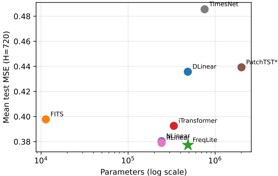
Accuracy vs. model size (L=336, averaged over datasets)
