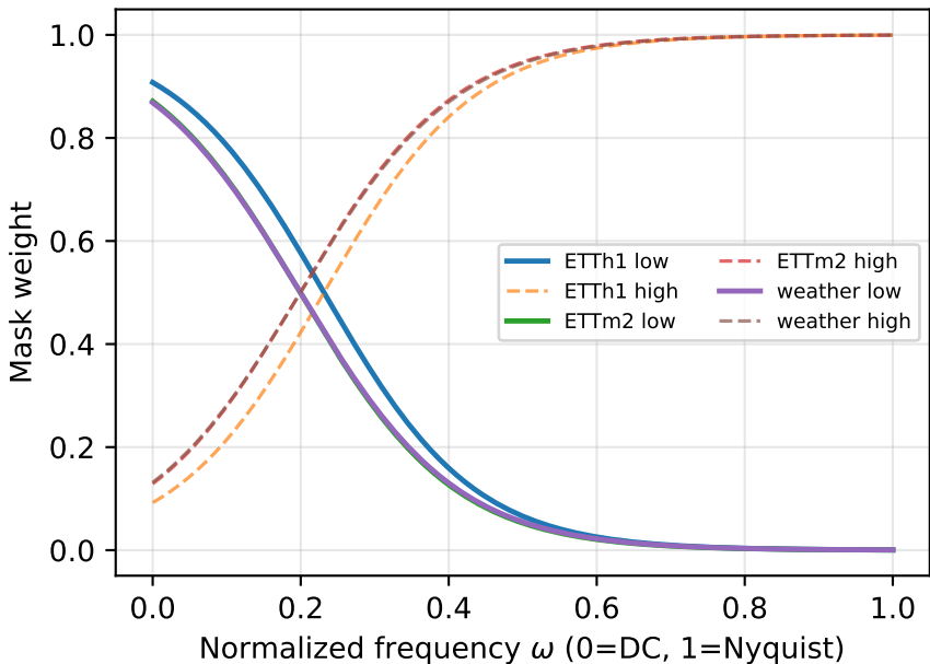
Learned spectral masks (L=336, H=720)
