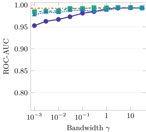
(a) In-distribution CV
