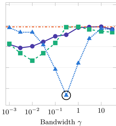
(b) Shifted test set
