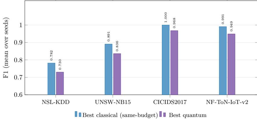
Figure 3: Best classical (same-budget) vs. best quantum F1 per dataset (mean over seeds). Tuned classical models lead on every dataset; the gap is largest on the discriminative datasets (NSL-KDD, UNSW-NB15) and smallest where the task is near-saturated (CICIDS2017, NF-ToN-IoT-v2, where every classical model exceeds 0.97).
