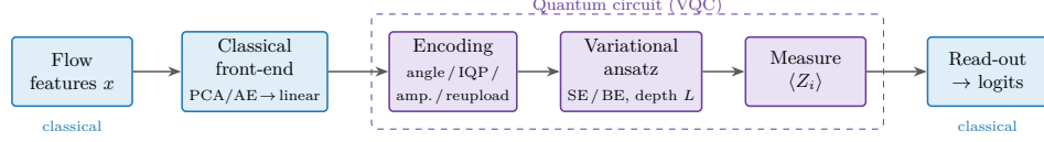
Figure 1: Hybrid quantum-classical classifier. A classical front-end compresses flow features to the per-qubit budget; a variational quantum circuit (encoding + ansatz + measurement) processes the encoded state; a classical read-out produces class logits. The quantum component is sandwiched between classical processing — the motivation for the attribution audit.
