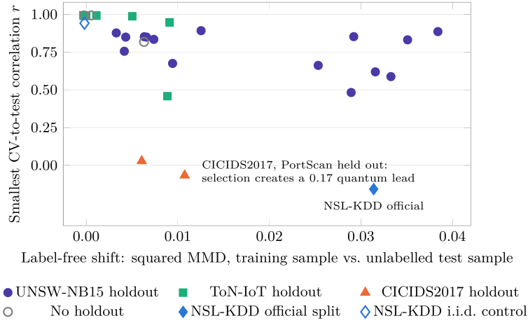
Figure 6: Label-free shift predicts when cross-validation stops ranking kernel settings. Each point is one kernel landscape (three kernels, 40 settings each): attack families held out of the 2,000-row training sample on UNSW-NB15, ToN-IoT and CICIDS2017 (filled), the same datasets without a holdout (open), and NSL-KDD’s official split and its i.i.d. control (diamonds). The horizontal axis needs no test labels. Across the 26 holdout runs, Spearman \rho = -0.61 (permutation p = 0.001 ). Generated from the result files.
