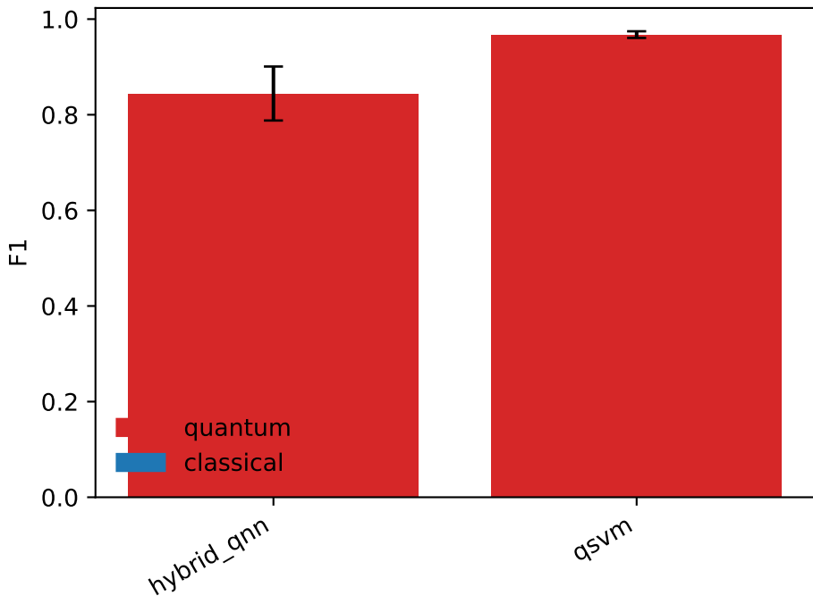
cicids: F1 by model (mean \pm std over seeds)
