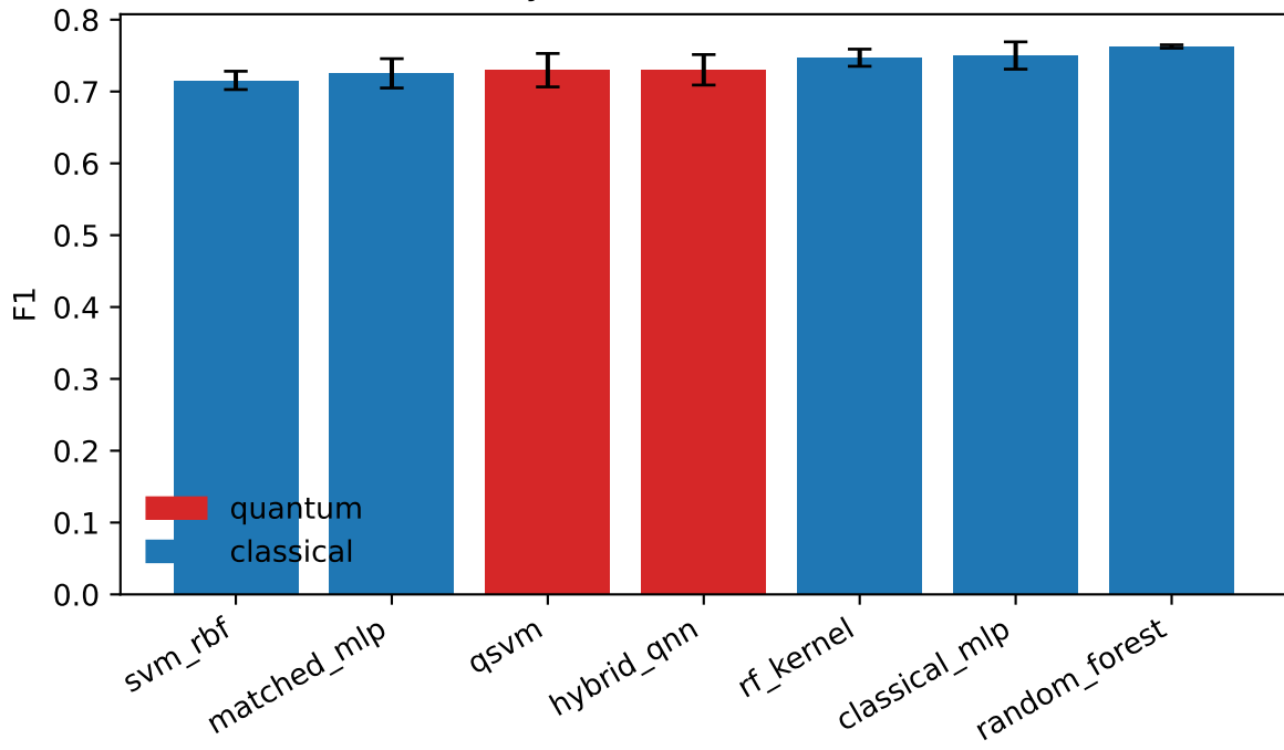
nsllkdd: F1 by model (mean \pm std over seeds)
