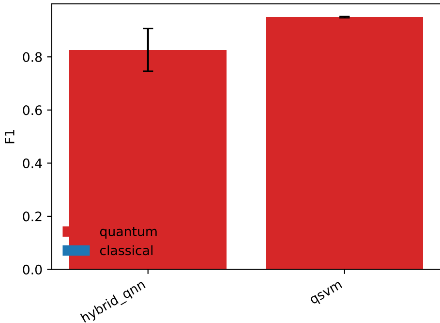
toniot: F1 by model (mean \pm std over seeds)
