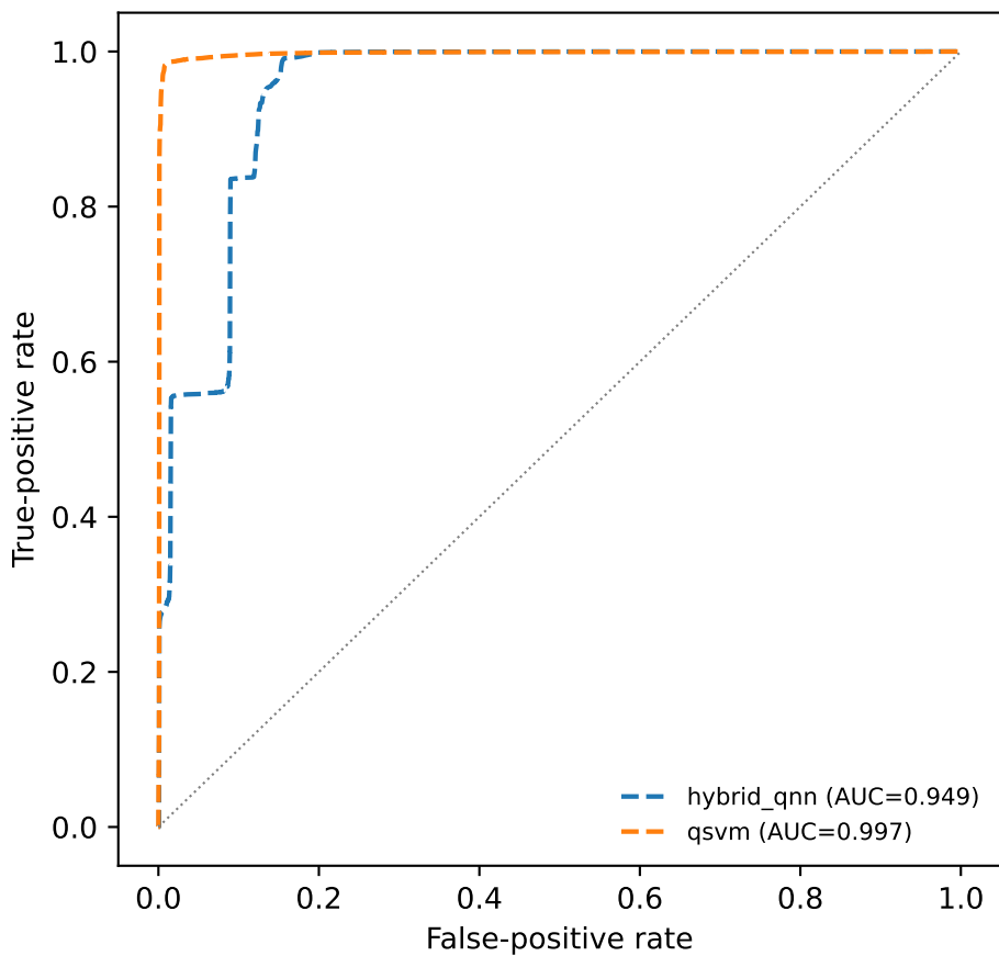
cicids: ROC curves
