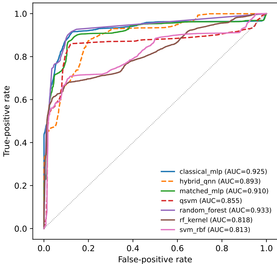
nsllkdd: ROC curves
