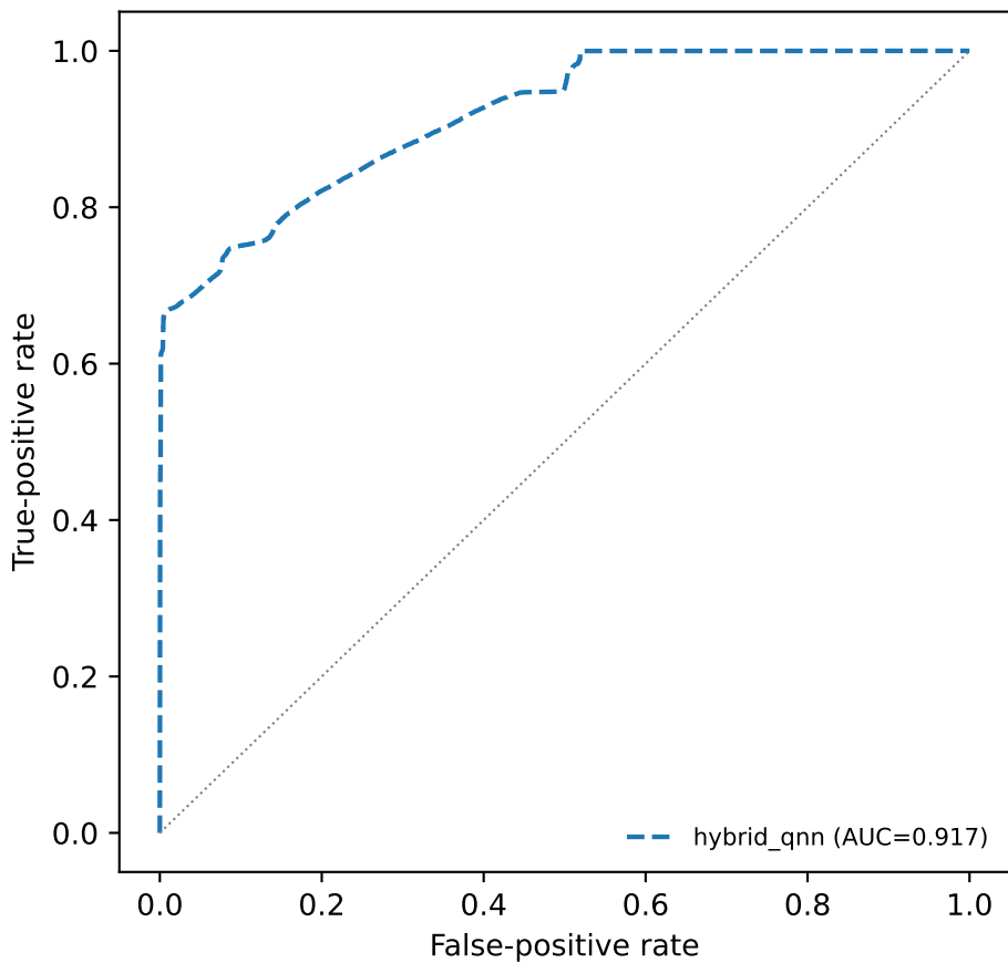
unsw: ROC curves
