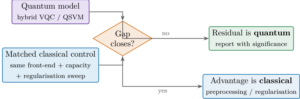
Figure 2: The attribution audit. Each quantum model is compared with a parameter-matched classical control sharing its front-end, plus a regularisation sweep. If a comparably-regularised classical model closes the gap, the apparent advantage is classical; any significant residual is attributed to the quantum circuit.
