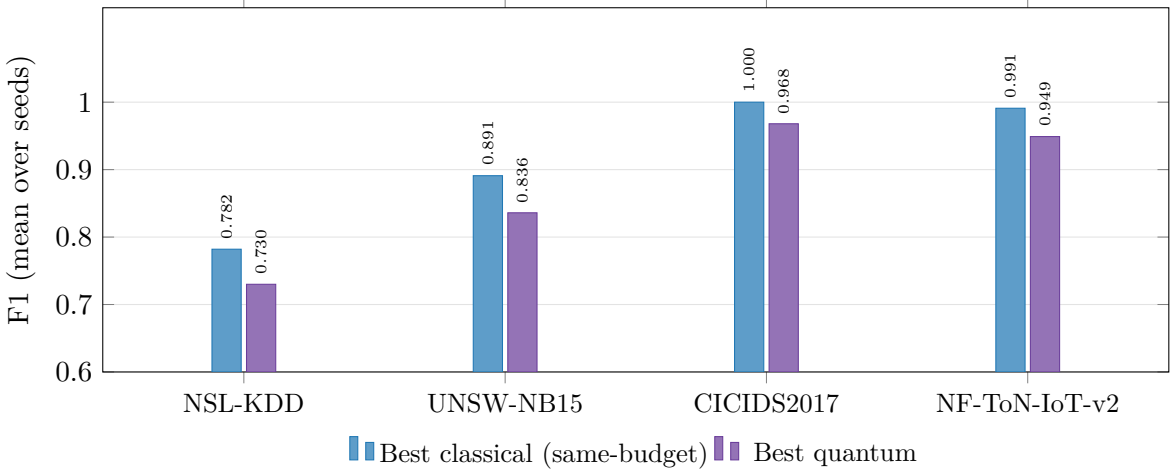
Figure 3: Best classical (same-budget) vs. best quantum F1 per dataset (mean over seeds). Tuned classical models lead on every dataset; the gap is largest on the discriminative datasets (NSL-KDD, UNSW-NB15) and smallest where the task is near-saturated (CICIDS2017, NF-ToN-IoT-v2, where every classical model exceeds 0.97).
