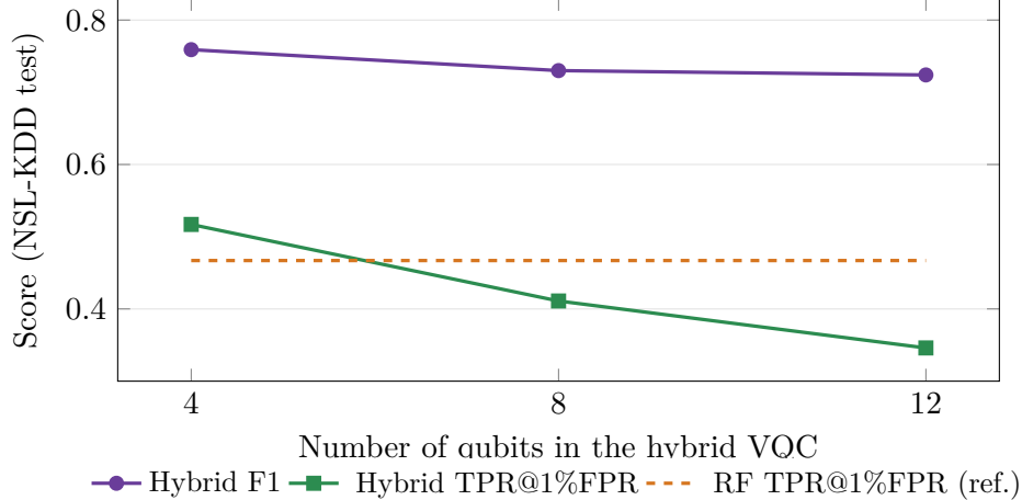
Figure 4: Qubit-count ablation of the hybrid VQC on NSL-KDD. Both F1 and the low-FPR detection rate decline with width — more qubits do not help on the shifted task. Crucially, only the small four-qubit circuit exceeds the best classical baseline’s TPR@1%FPR (Random Forest, dashed reference at 0.467); the advantage vanishes by twelve qubits, consistent with an implicit-regularisation mechanism rather than raw expressivity.
