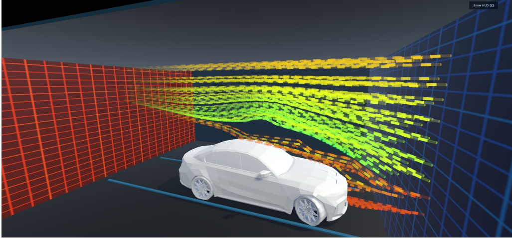
Vertical streamline pass highlighting roof flow, ground interaction, and wake rise.
