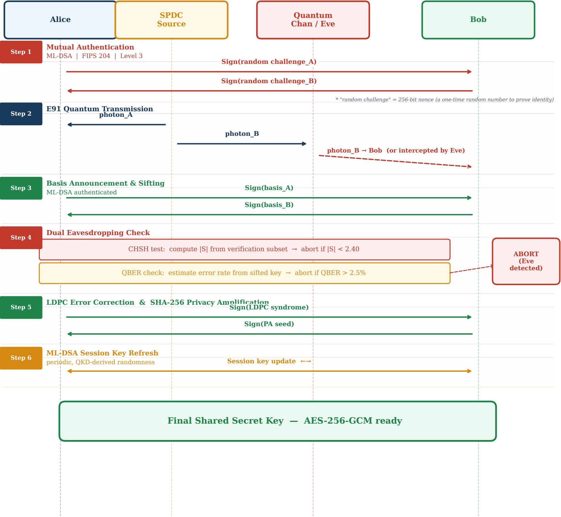
Fig. 2 — Hybrid E91 + ML-DSA Protocol Sequence Diagram
