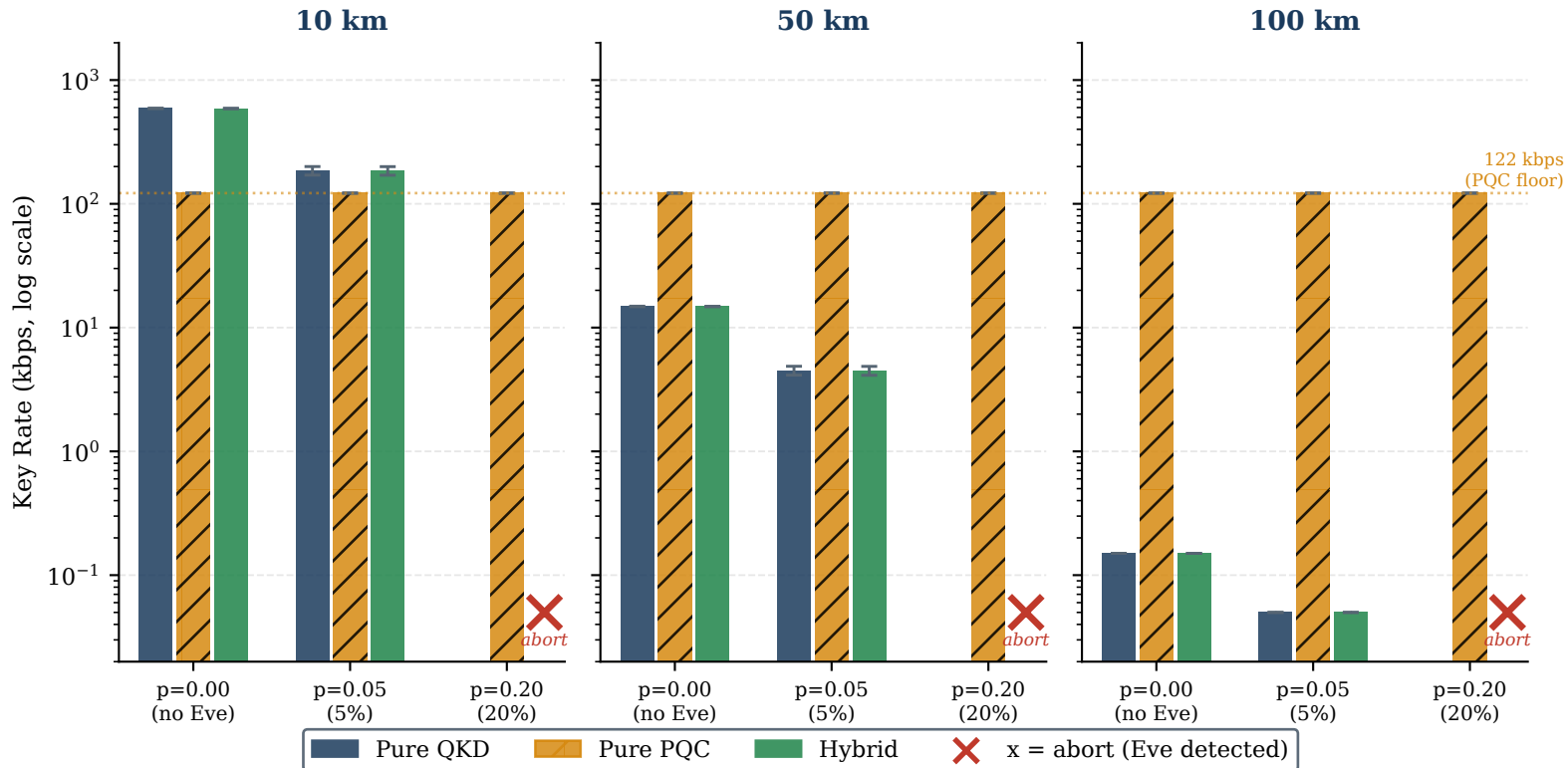
Fig. 3 — Secret Key Rate: Pure QKD vs. Pure PQC vs. Hybrid
