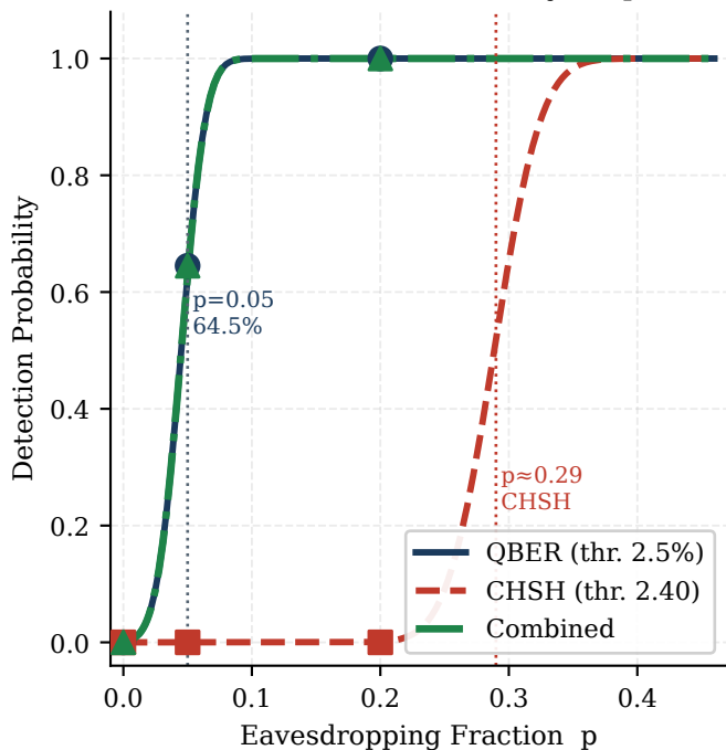
(a) Detection Probability vs. p
