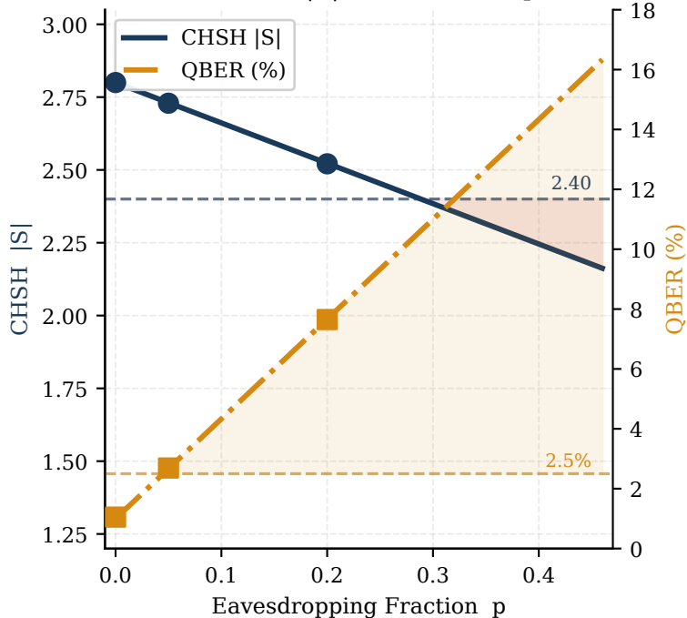
(b) CHSH |S| and QBER vs. p
